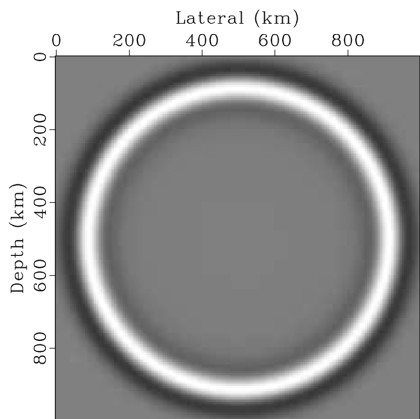
Forward: t=0.28\text{s}
