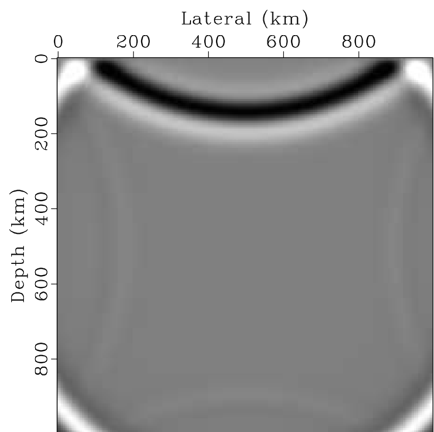
Forward: t=0.4\text{s}
