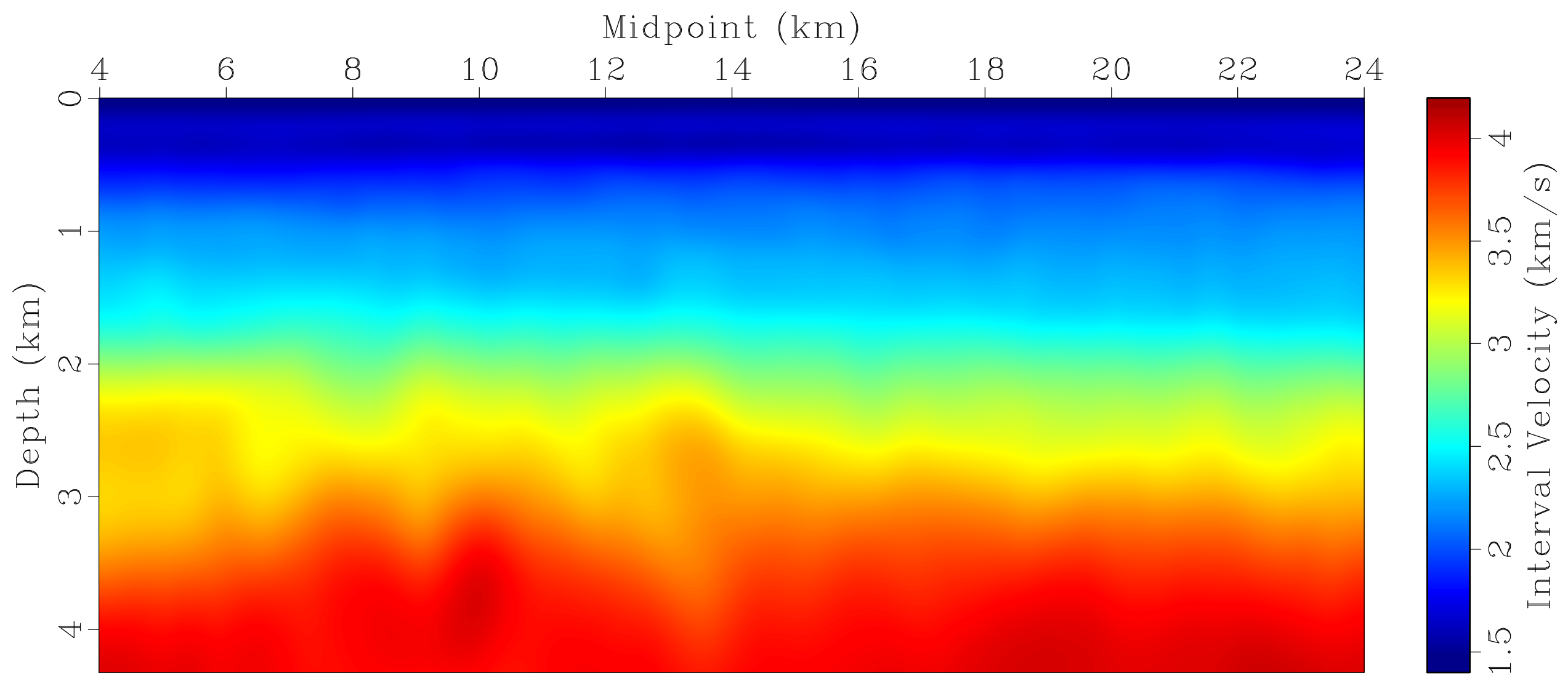
Continuation Model Interval Velocity in Depth
