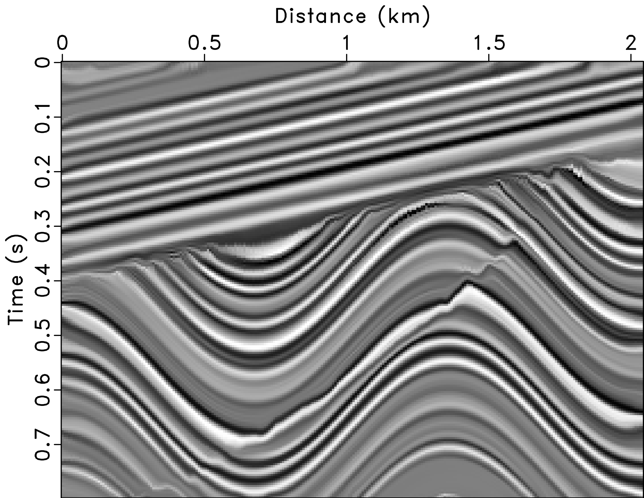
Inverse RT-seislet Transform (1%)
