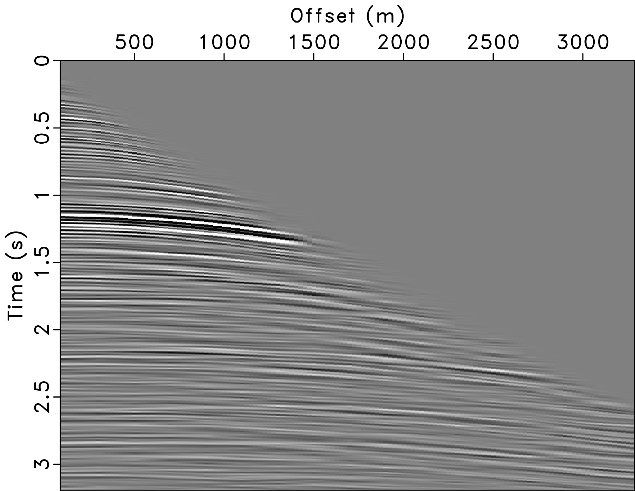
Denoising result
