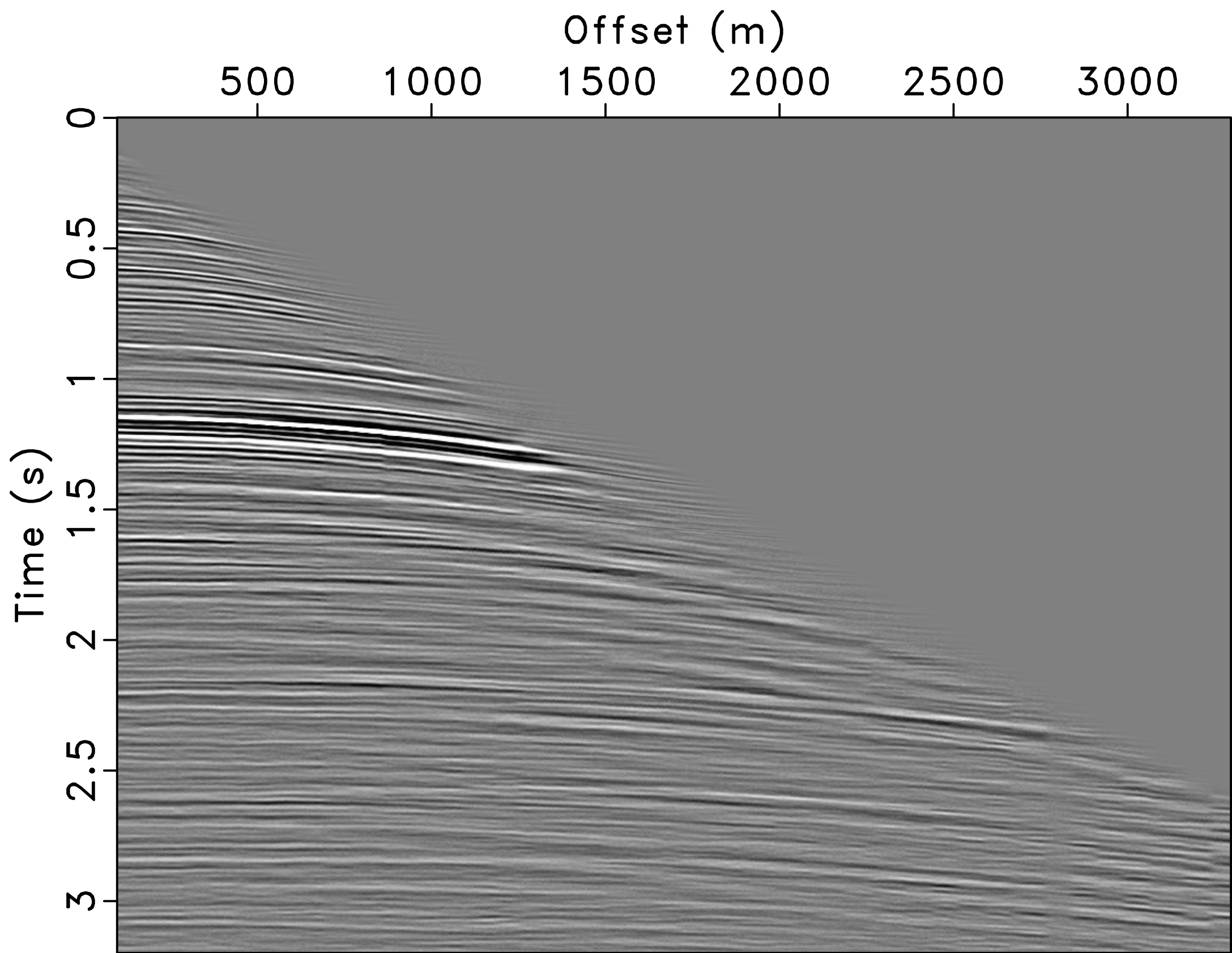
Interpolated shot gather
