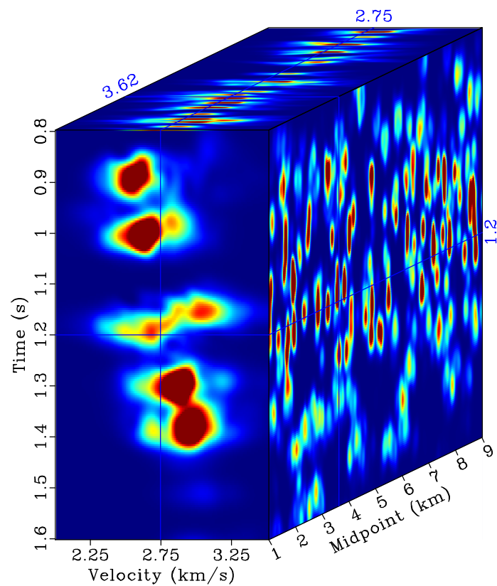
Combined Weights
