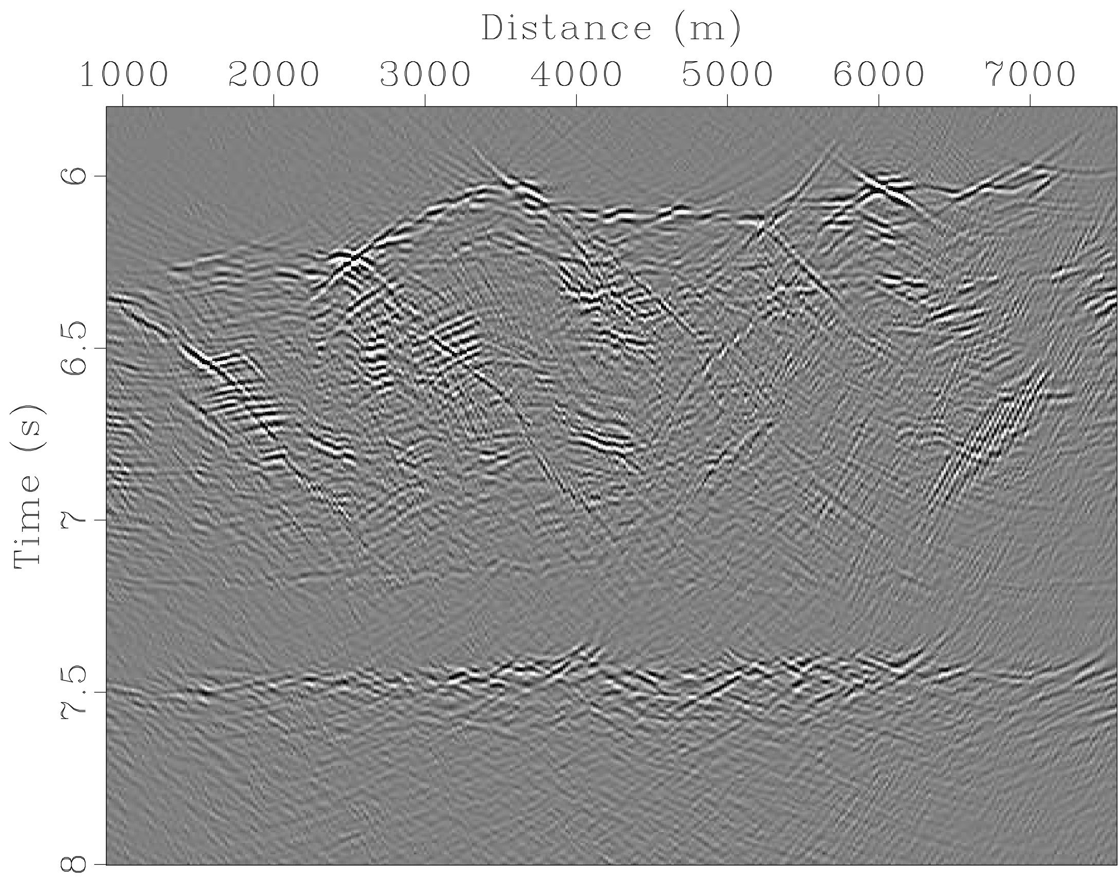
Diffraction Image
