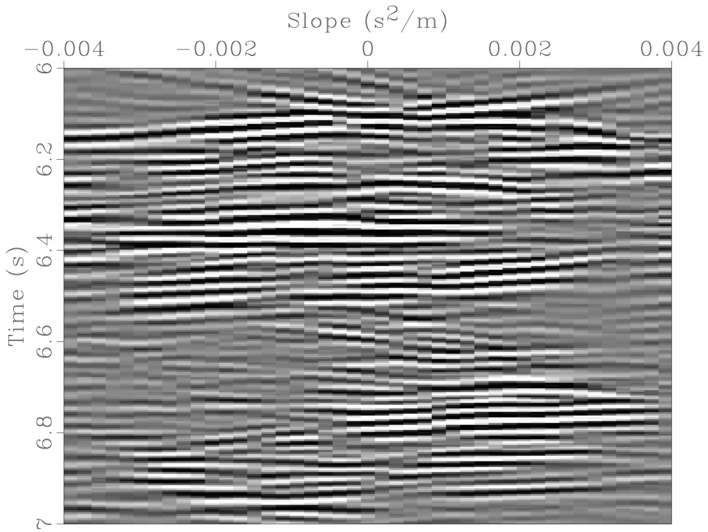
Slope Gather for Migration Velocity
