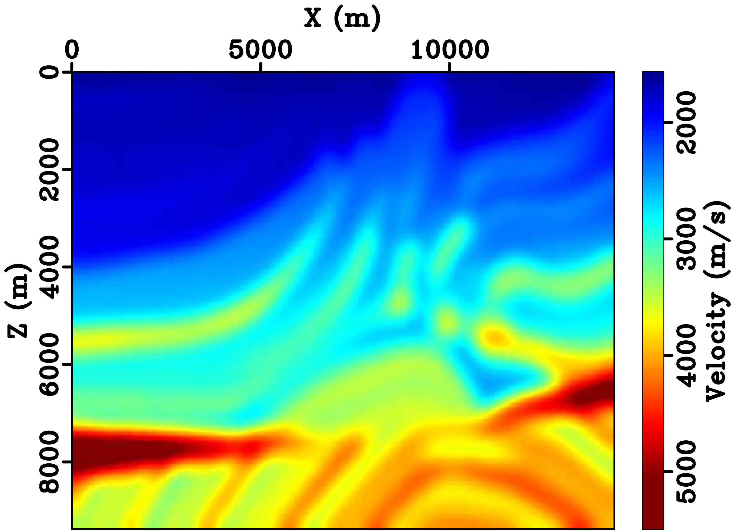
Marmousi Model
