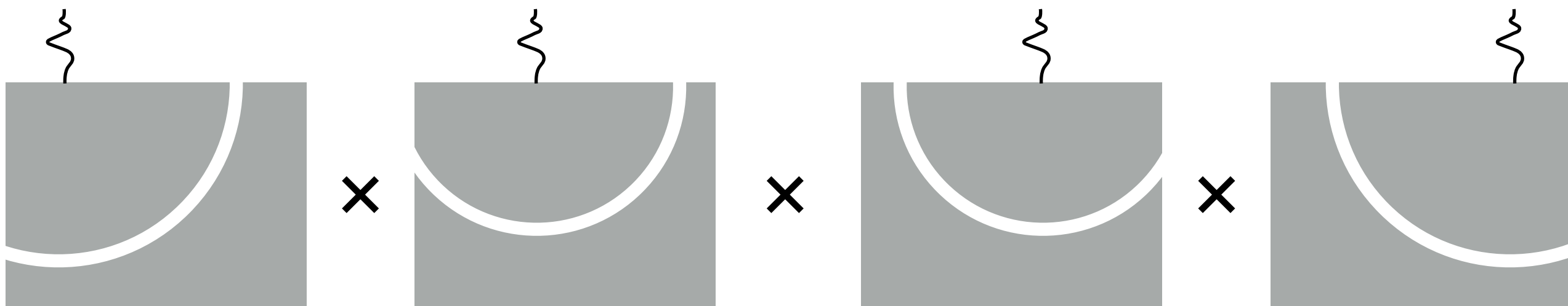
Cross-correlation imaging condition
