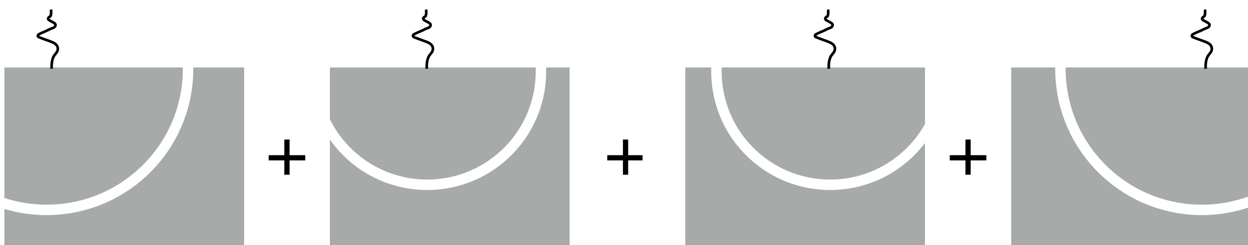
Time-reversal imaging condition
