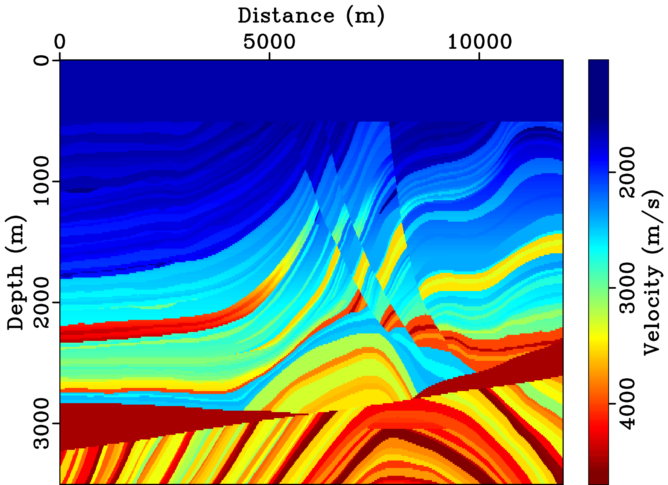
Marmousi Velocity Model
