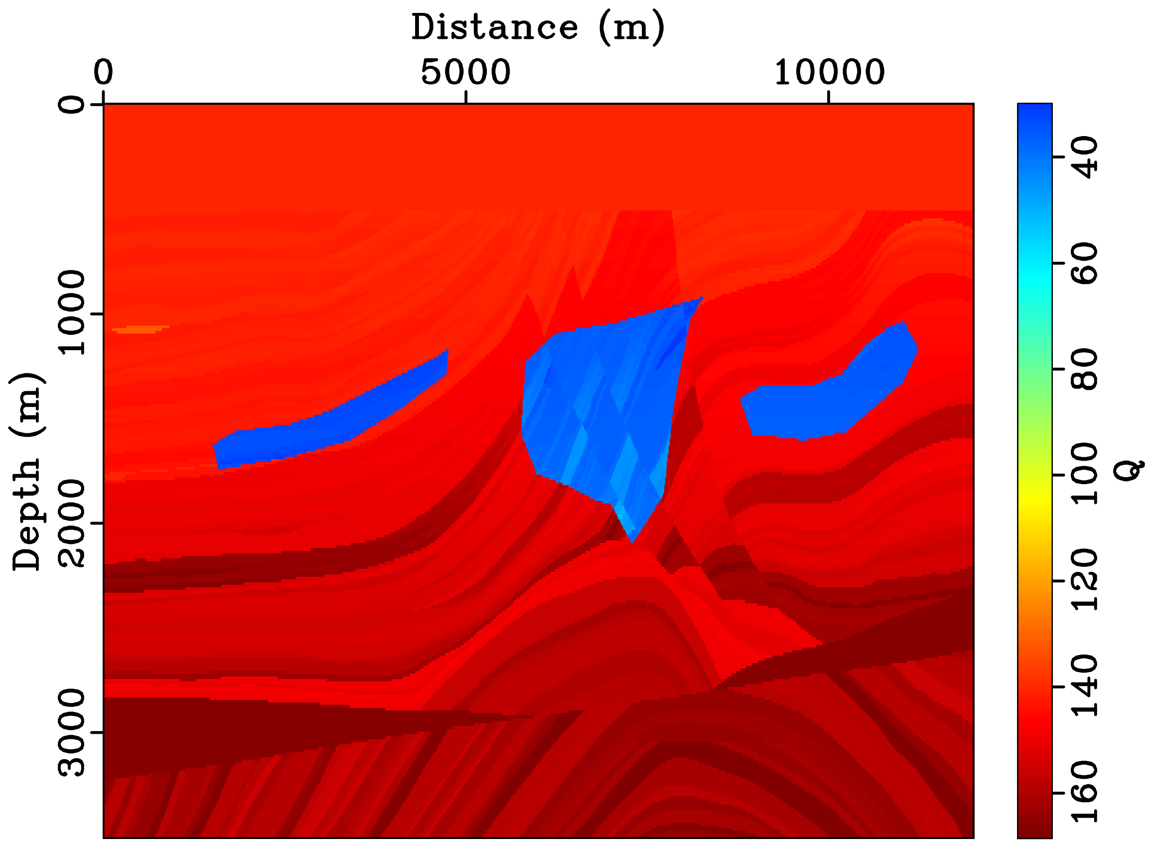
Marmousi Attenuation (Q) Model
