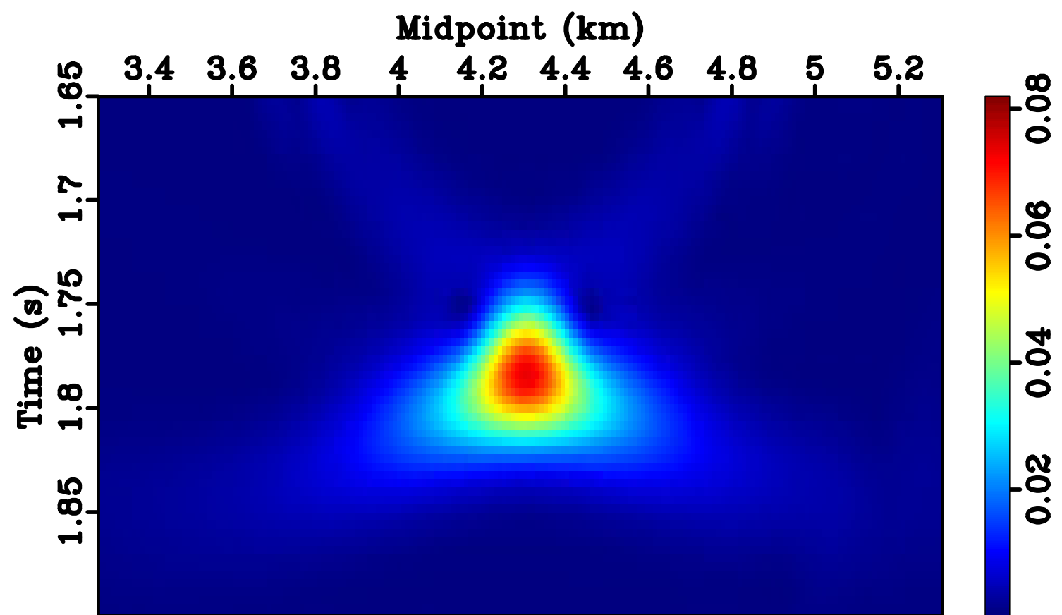
Focus of migrated diffraction (1D)
