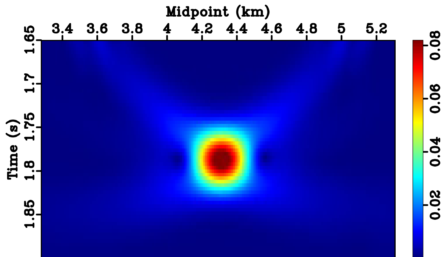
Focus of migrated diffraction (Proposed)
