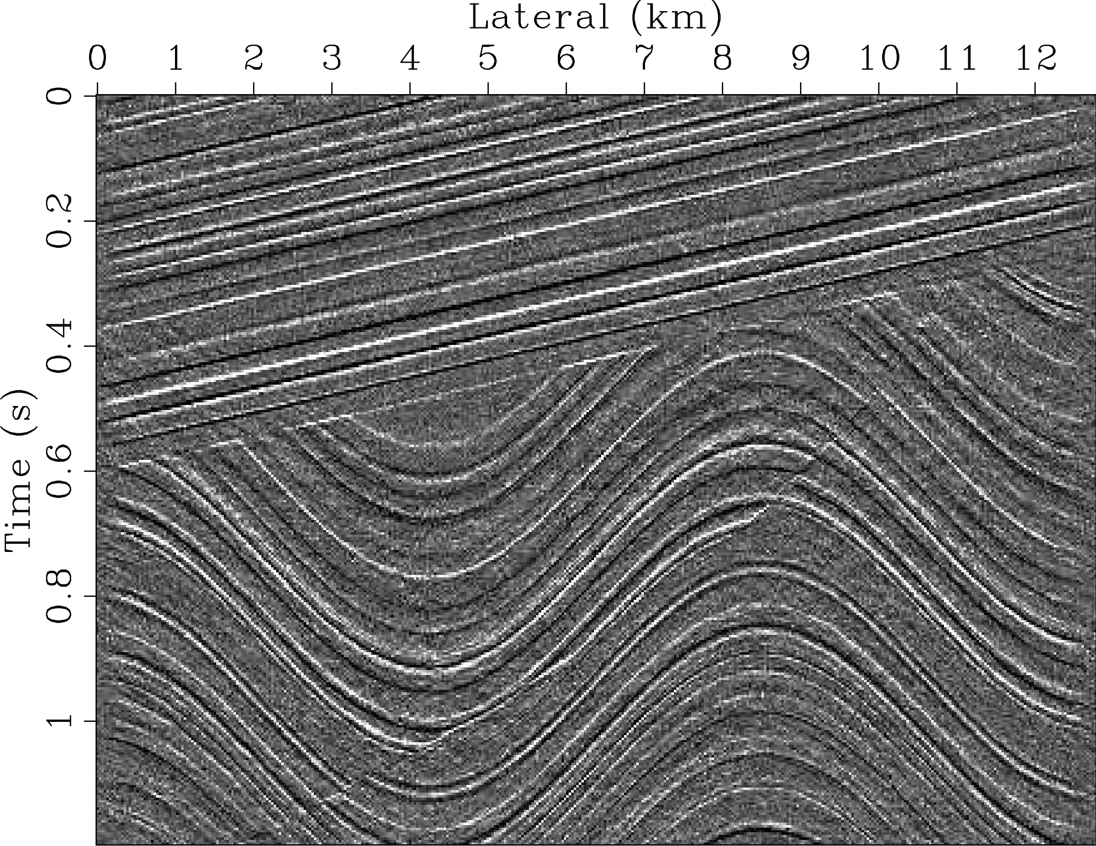
Denoised image
