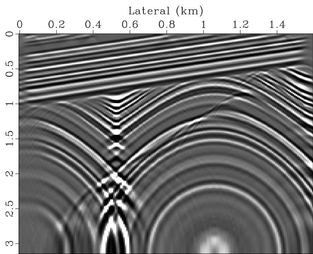
Transformation to Chebyshev grid
