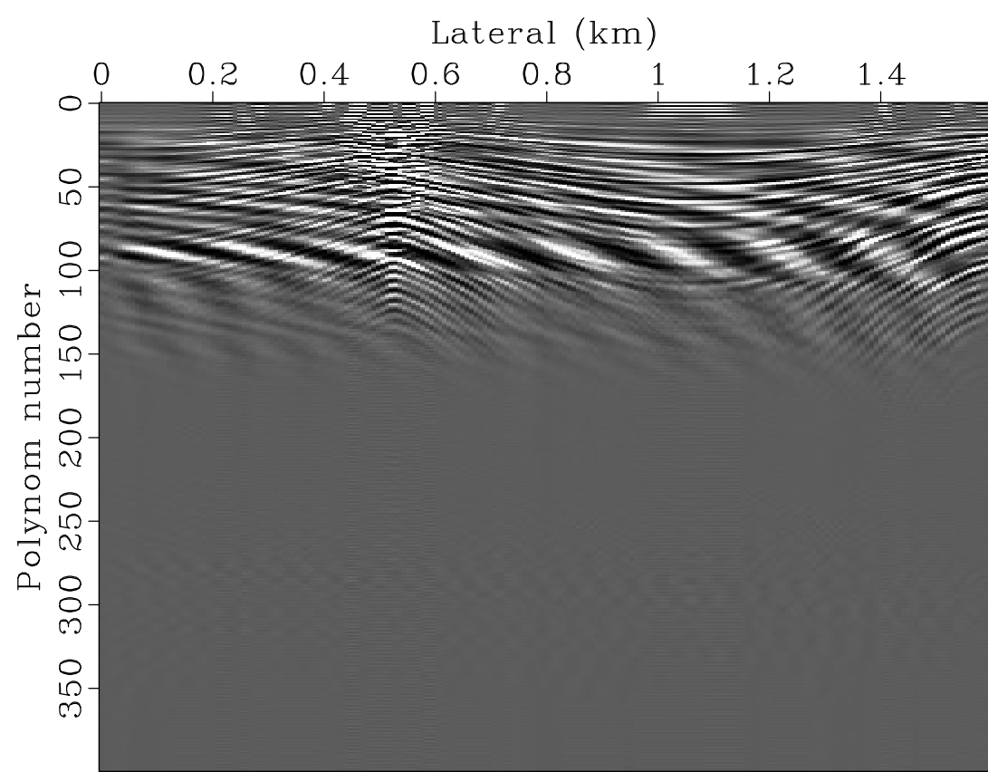
Chebyshev transform
