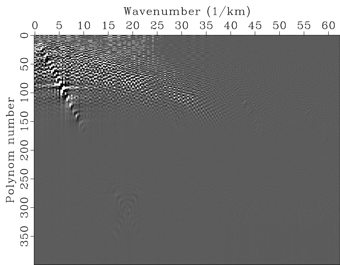
Chebyshev-Cosine FT
