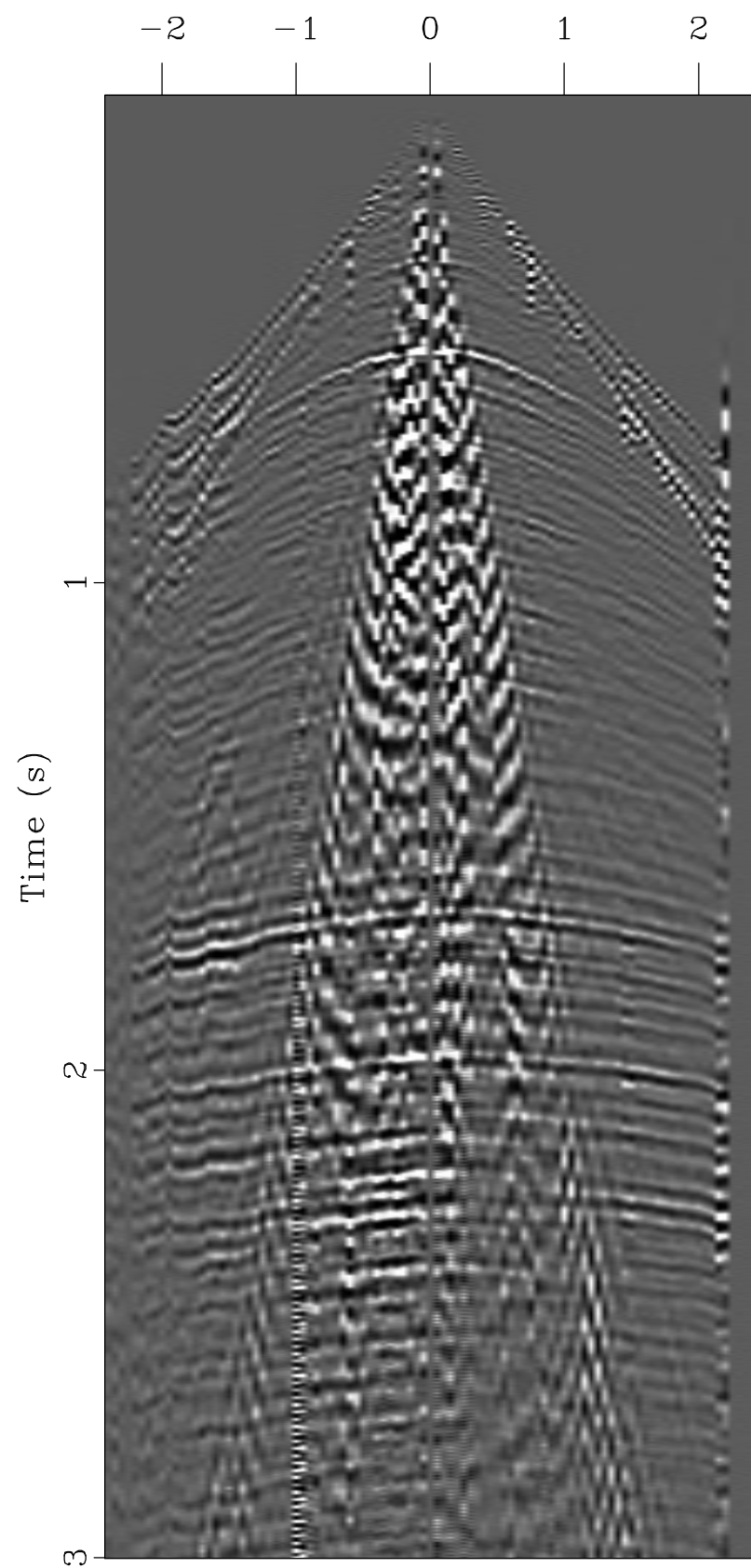
Shot Gather
