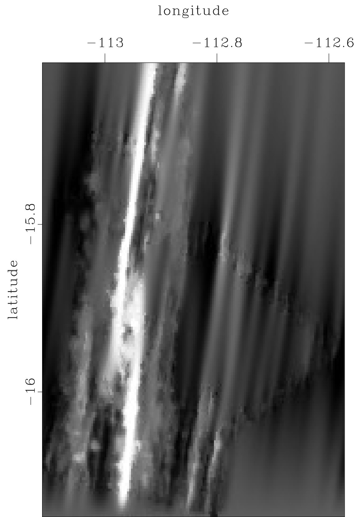
Data-space: 20 iterations
