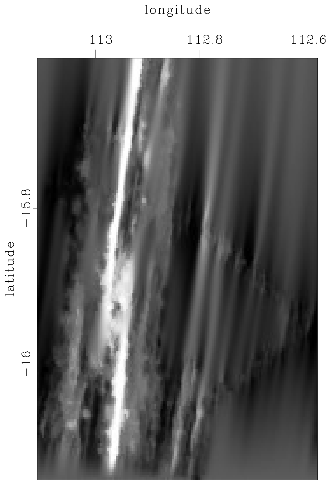
Data-space: 200 iterations
