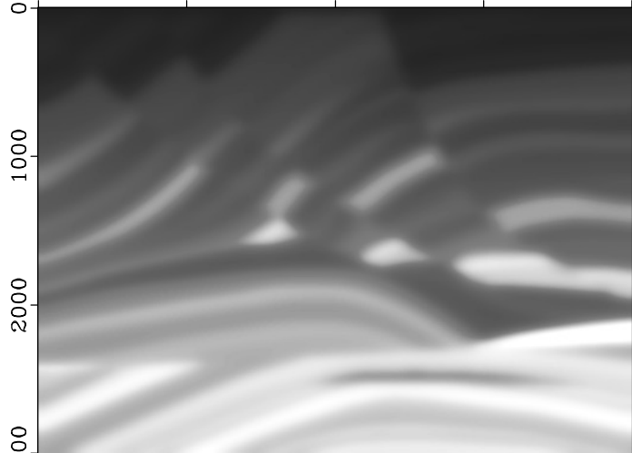
Smoothed Marmousi Model
