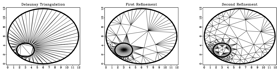
Figure A-8: An illustration of Rivara's refinement algorithm. The left plot shows an input to the algorithm: a valid Delaunay triangulation with "skinny" triangles. Two other plots show successive applications of the refinement algorithm.
