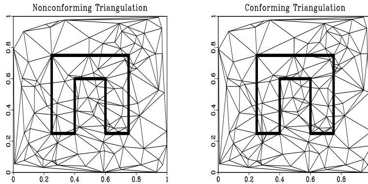
Figure A-4: An illustration of conforming triangulation. The left plot shows a triangulation of 500 random points; the triangulation in the right plot is conforming to the embedded boundary. Conforming triangulation is a genuine Delaunay triangulation, created by adding additional nodes to the original distribution.
