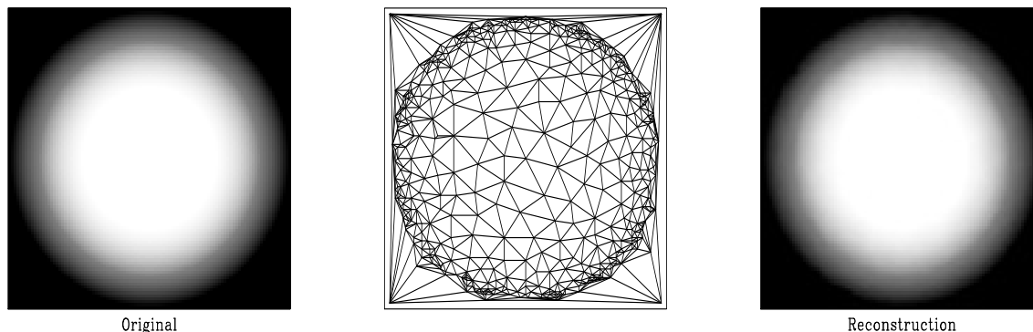
Figure A-5: Illustration of Garland's algorithm for triangulation of height fields. The left plot shows the input image of a sphere, containing 100 by 100 pixels. The middle plot shows 500 pixels, selected by the algorithm and triangulated. The right plot is the result of local plane interpolation of the triangulated surface.
