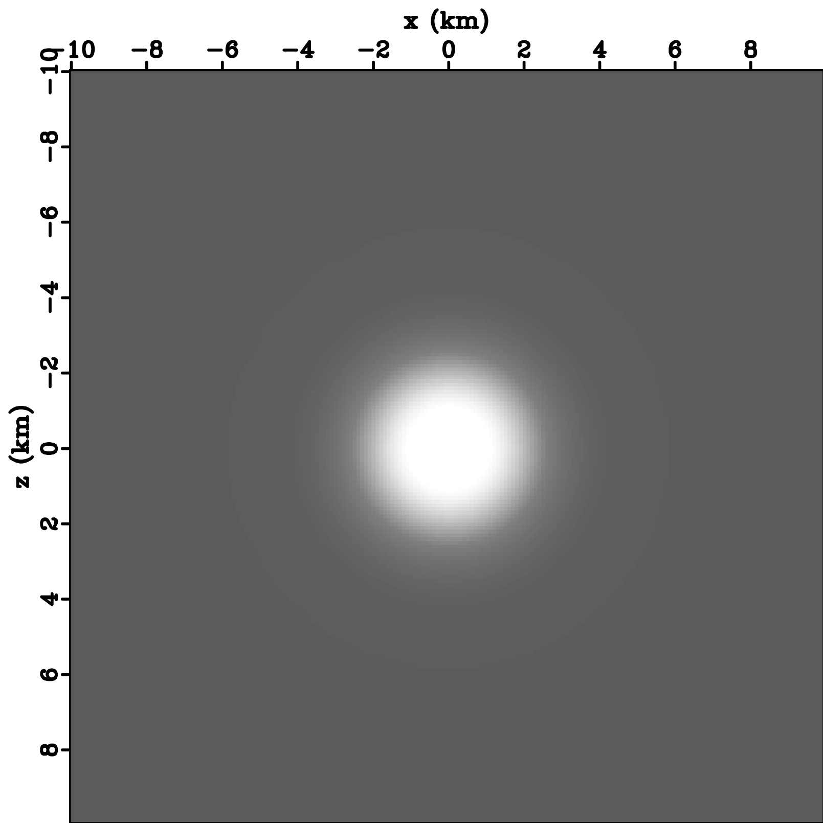
2D Gaussian
