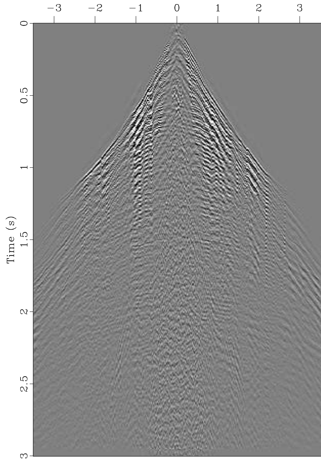
Ground-roll Removal
