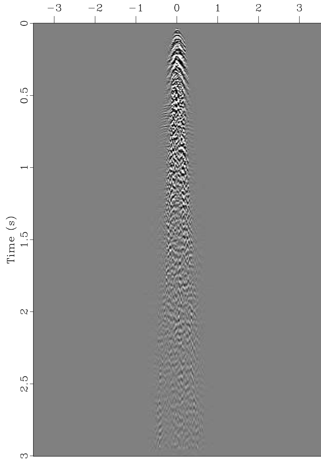
Ground-roll 198
