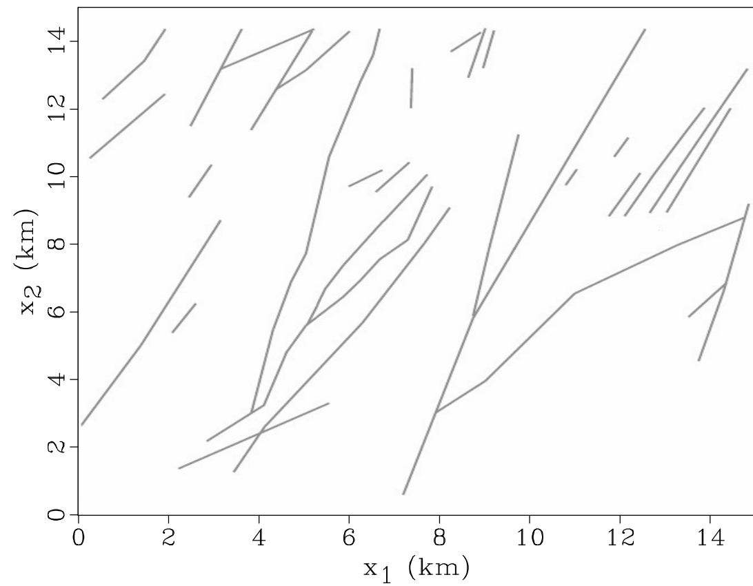
a) Fault Map
