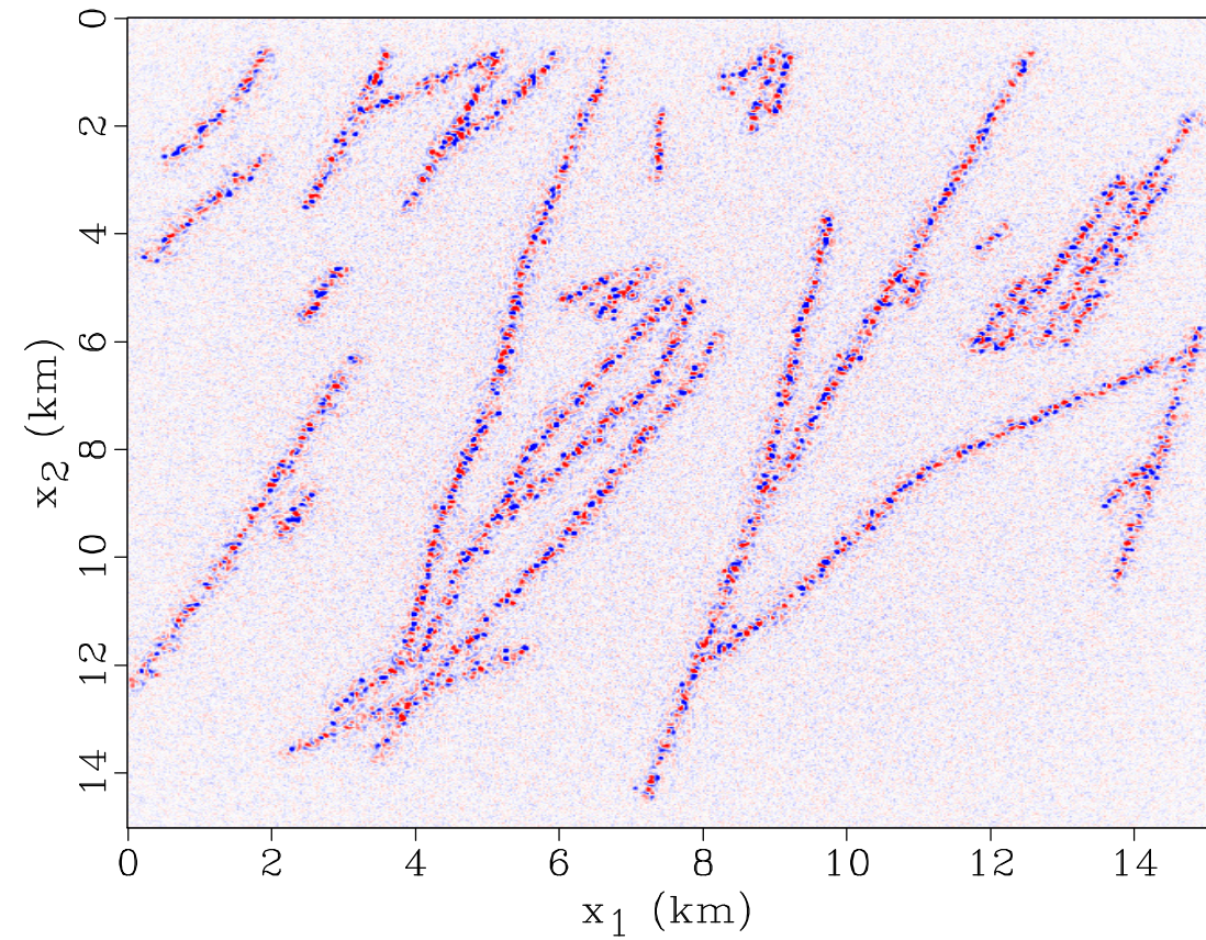
d) Anisotropic Velocity Continuation
