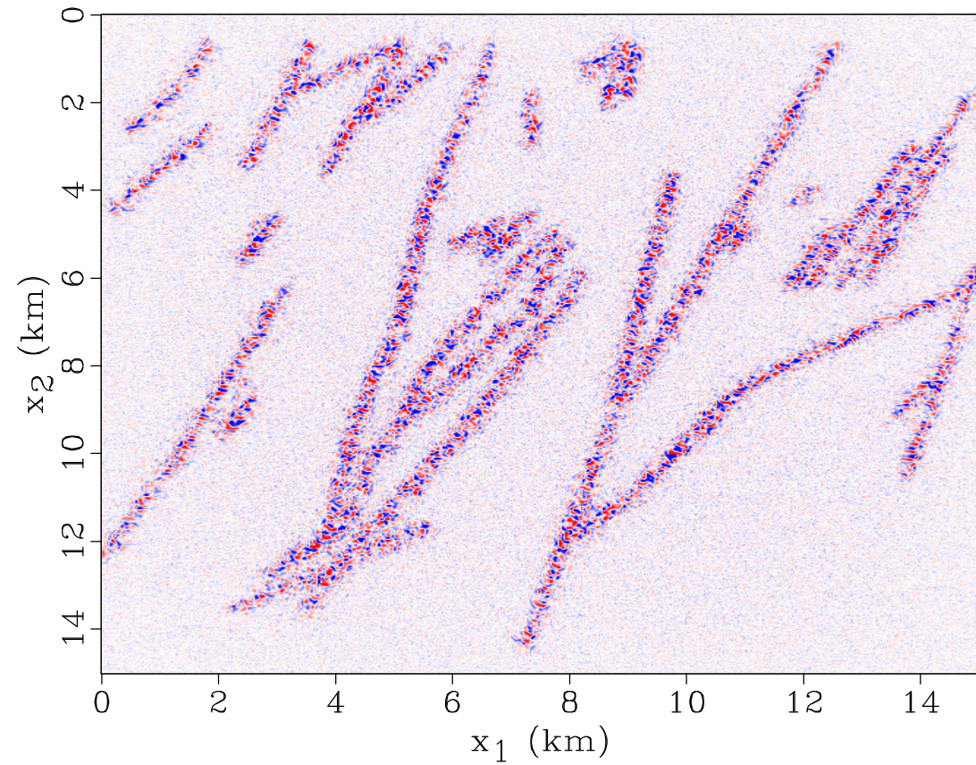
c) Isotropic Velocity Continuation
