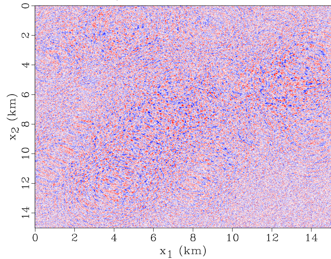
b) Fault Diffractions
