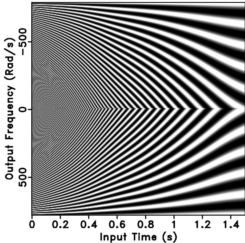
Inverse NMO Matrix
