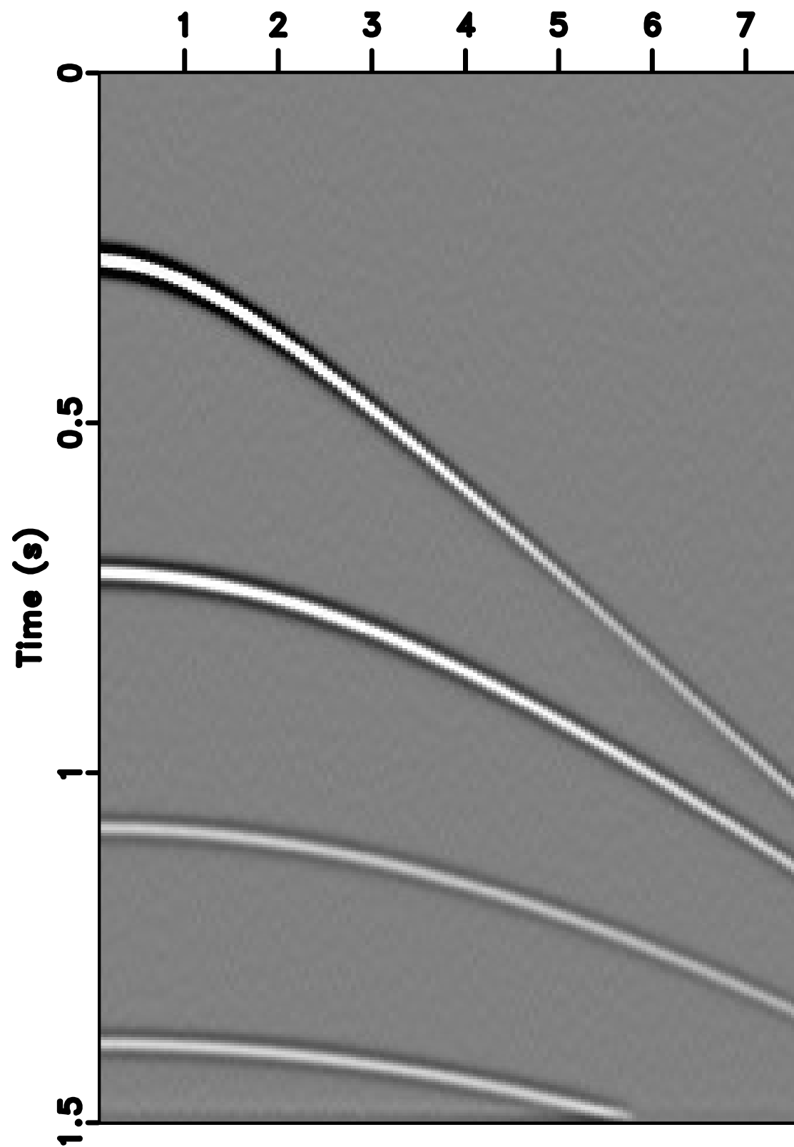
CMP Gather
