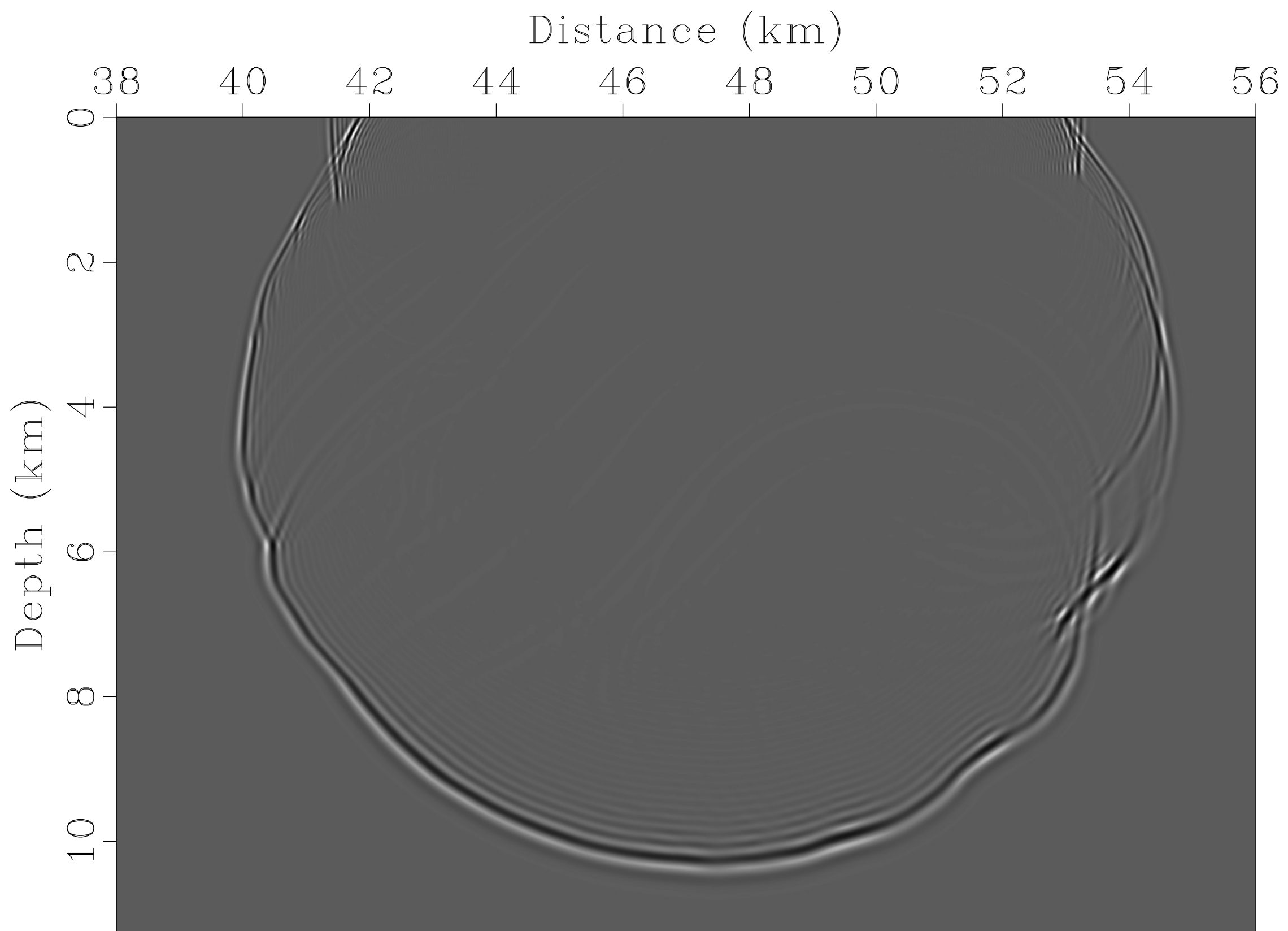
Snapshot in the BP 2D TTI model
