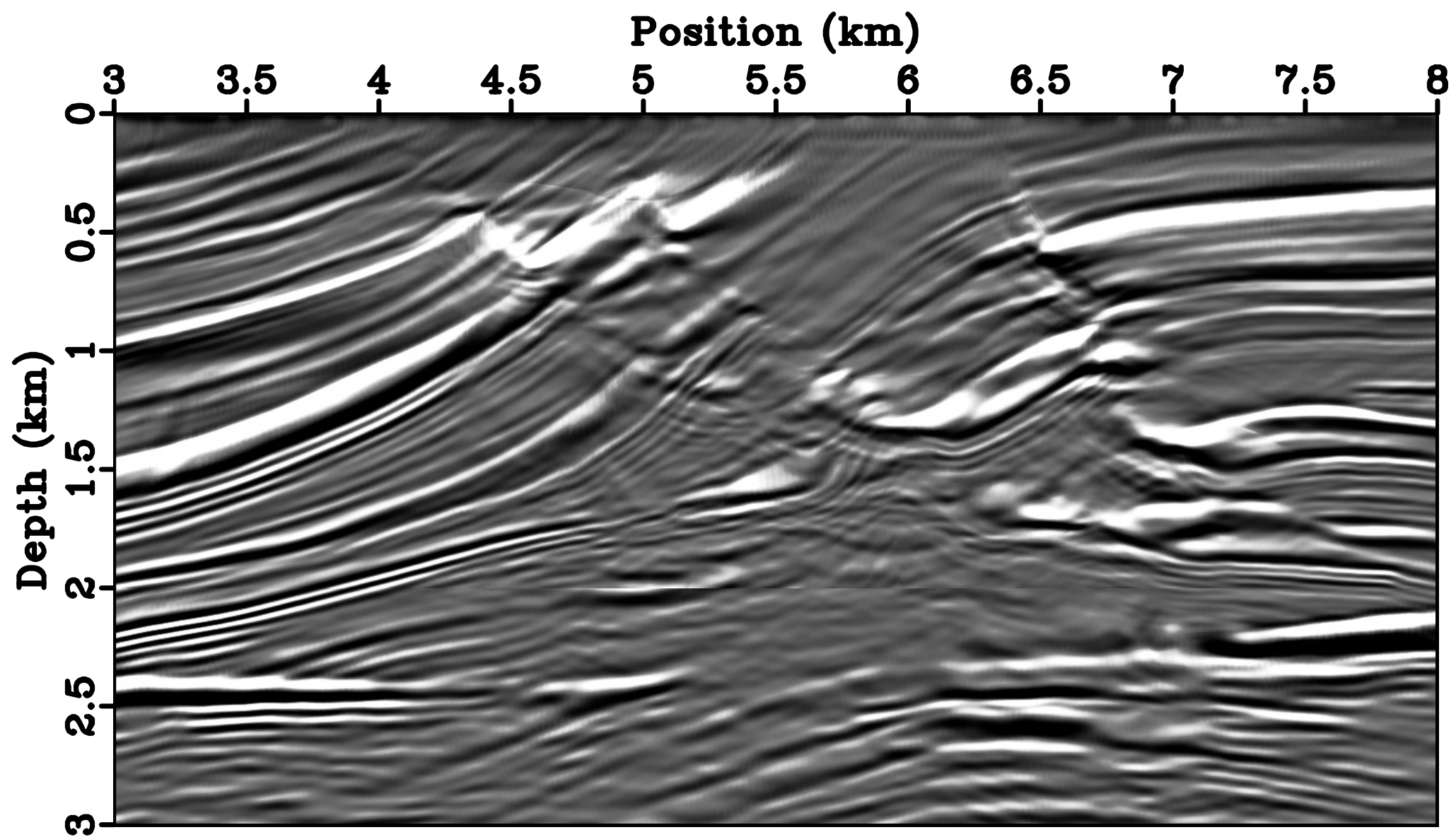
Recursive 3 steps
