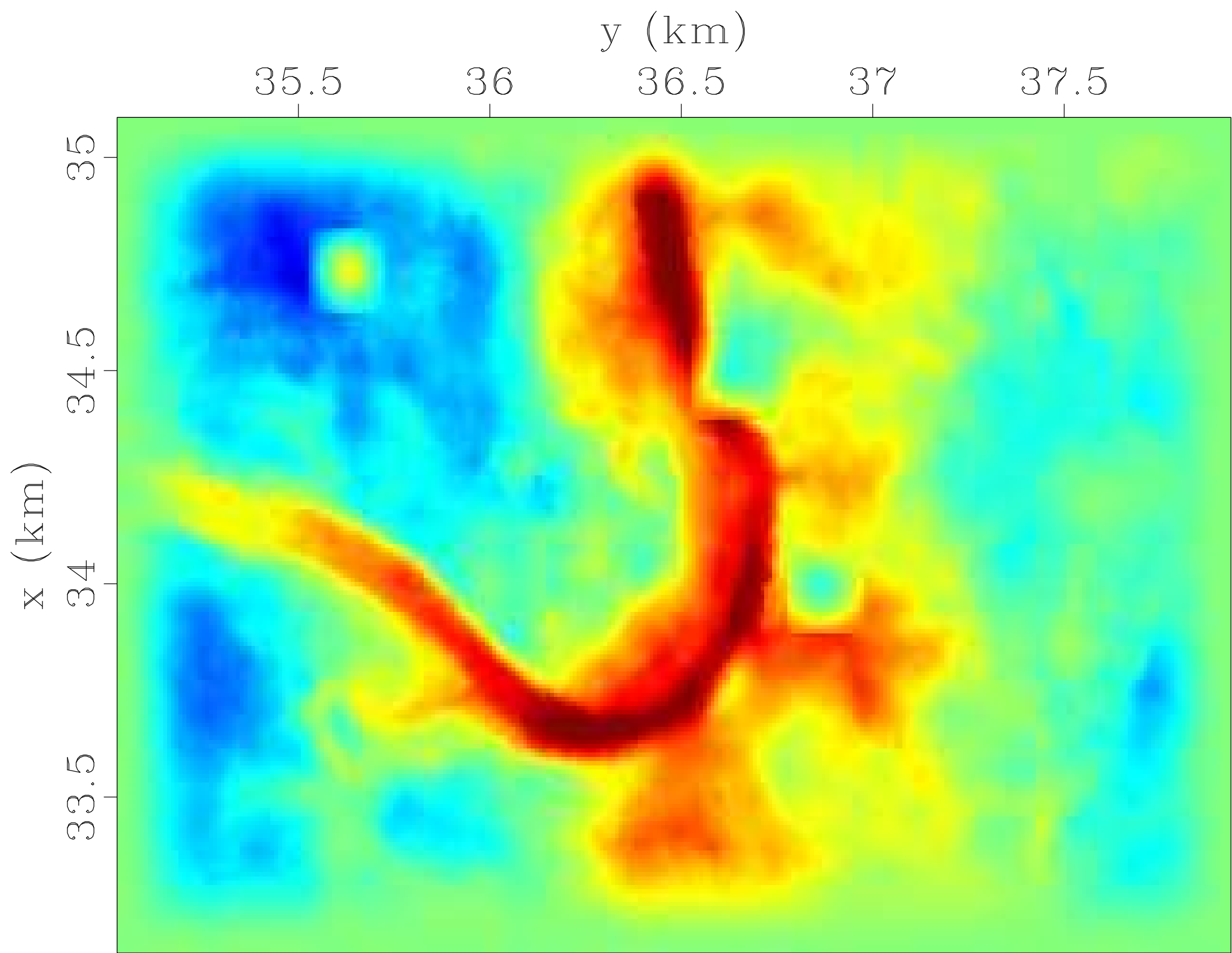
POCS interpolation (5 iterations)
