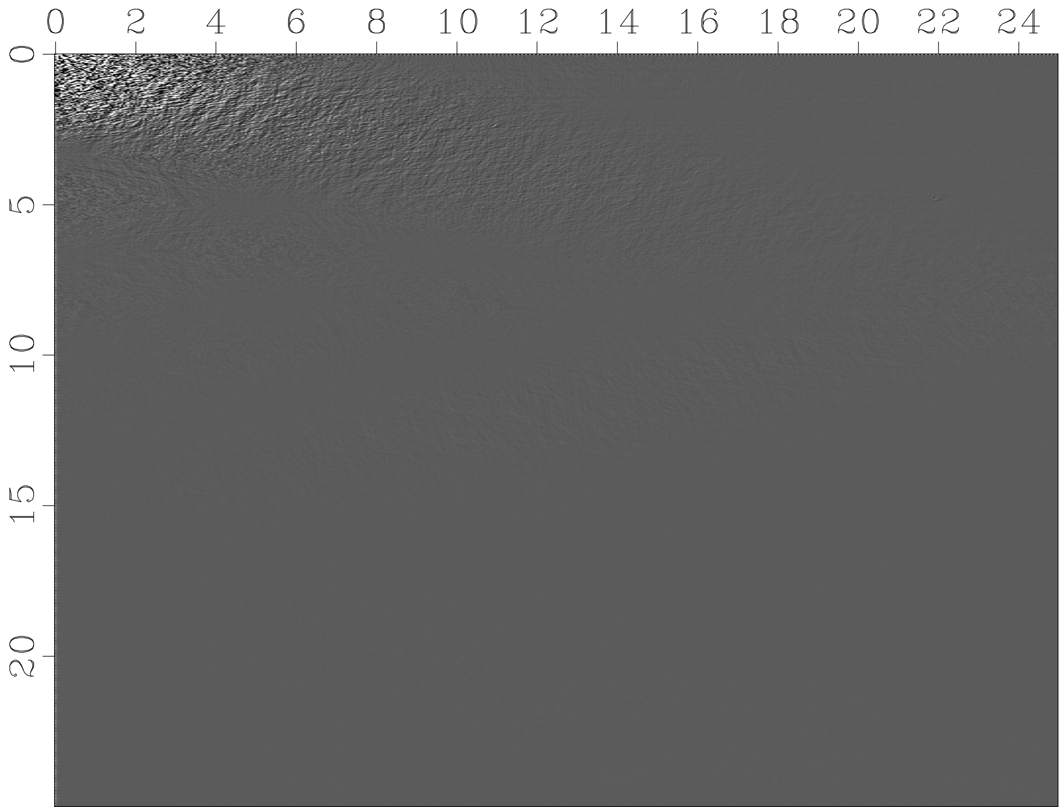
Cosine Fourier Transform
