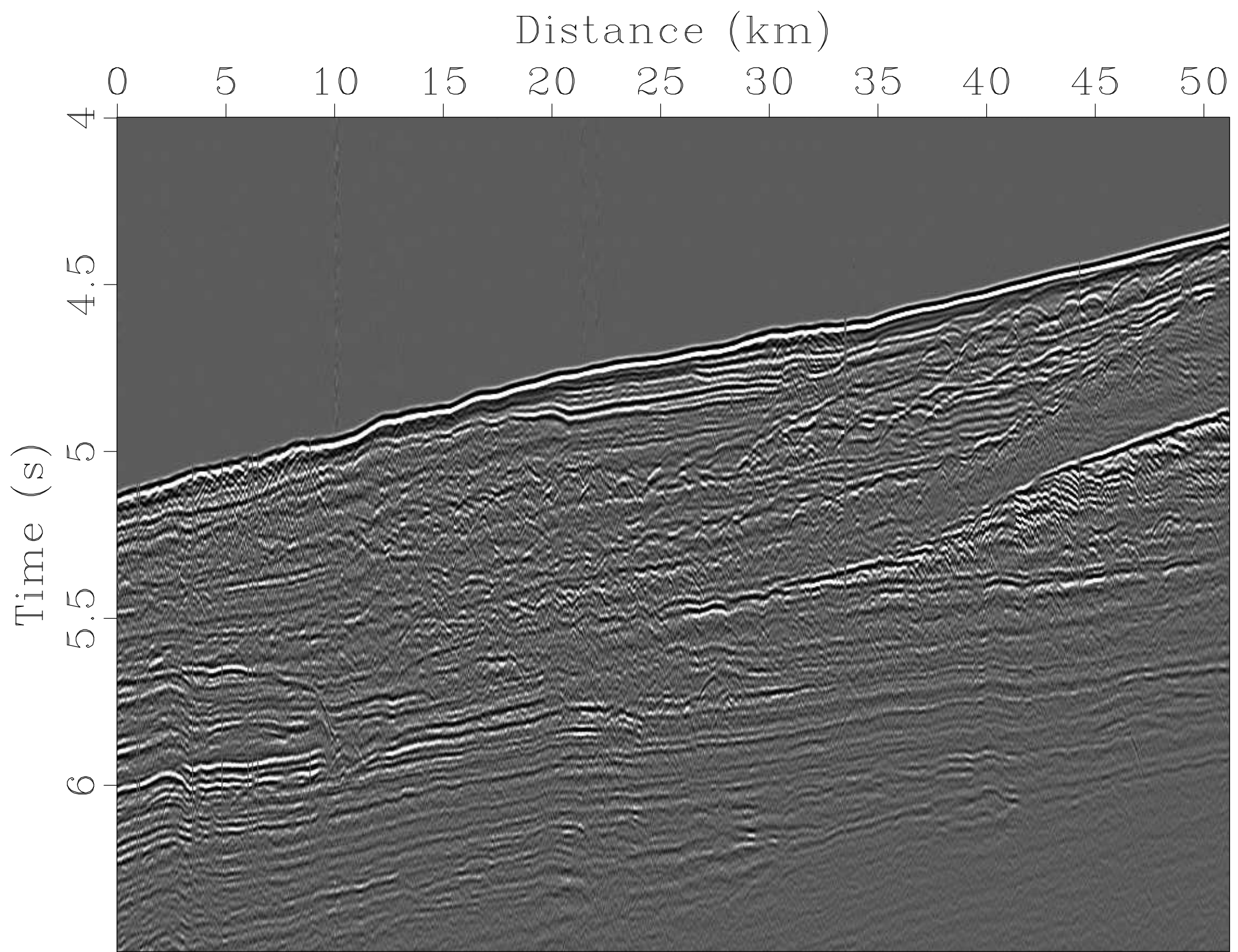
Near Offset Section
