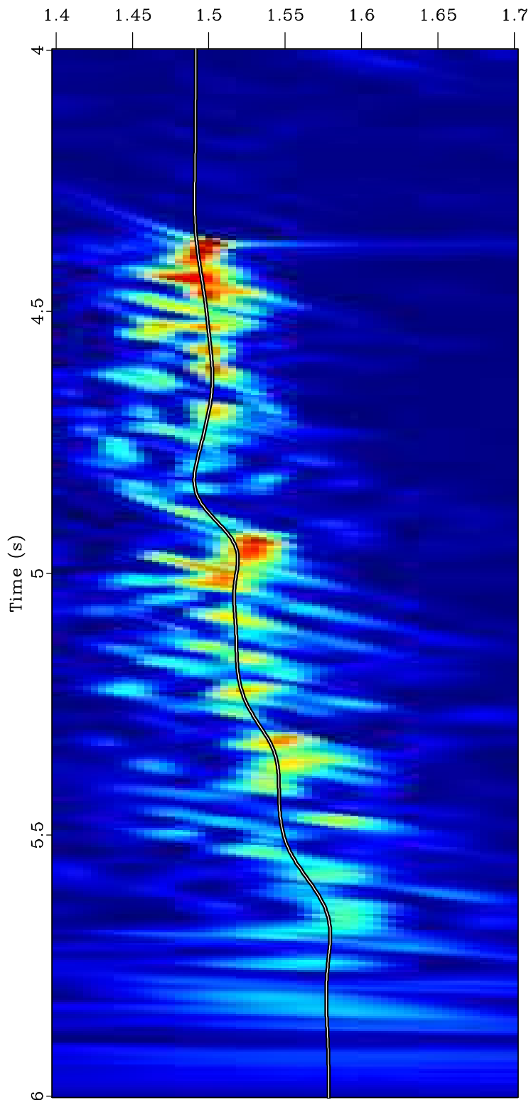
Velocity Scan
