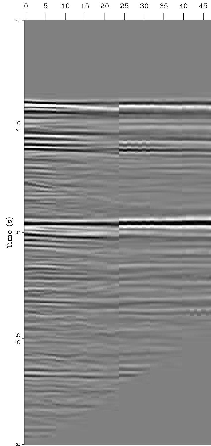
Normal Moveout
