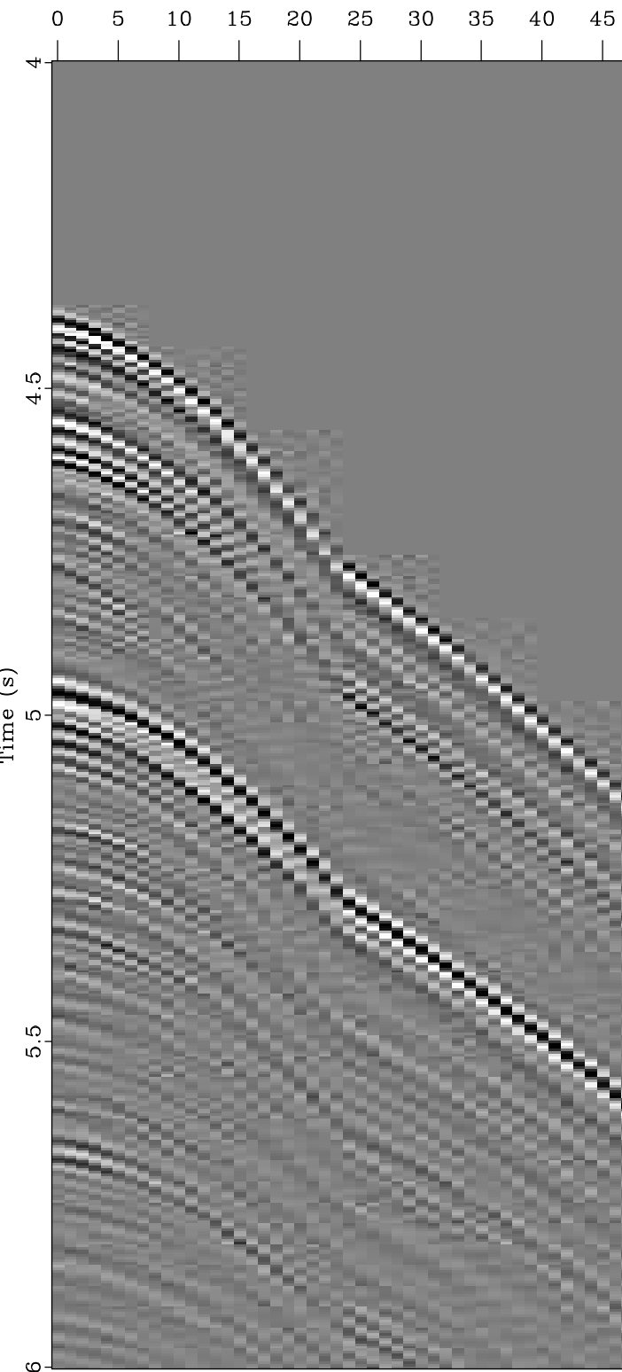
CMP gather
