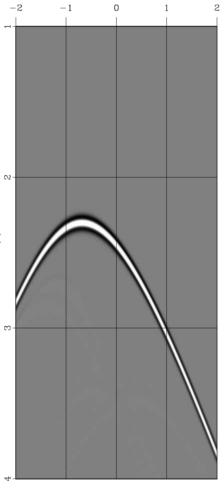
0 km Depth
