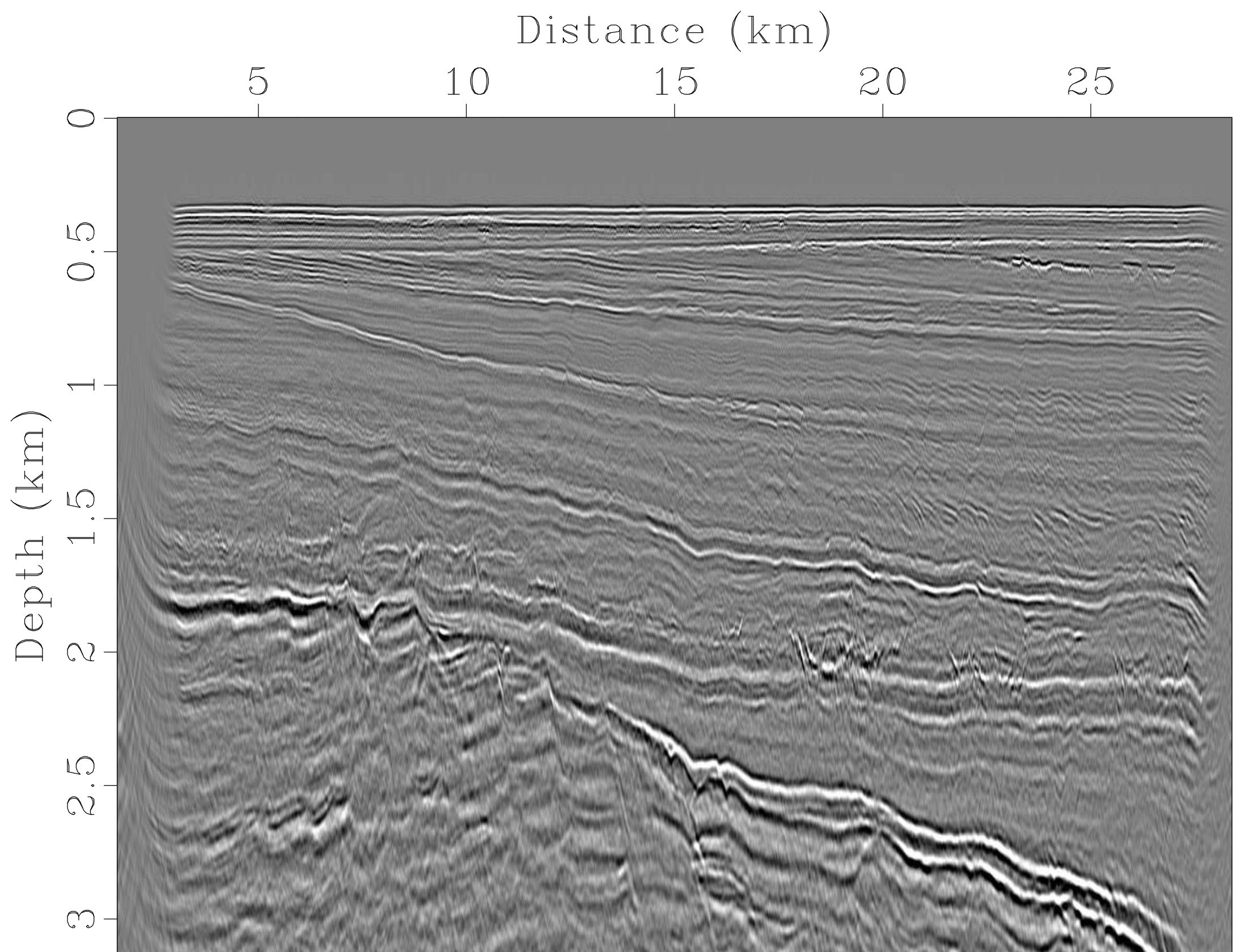
Post-Stack Depth Migration
