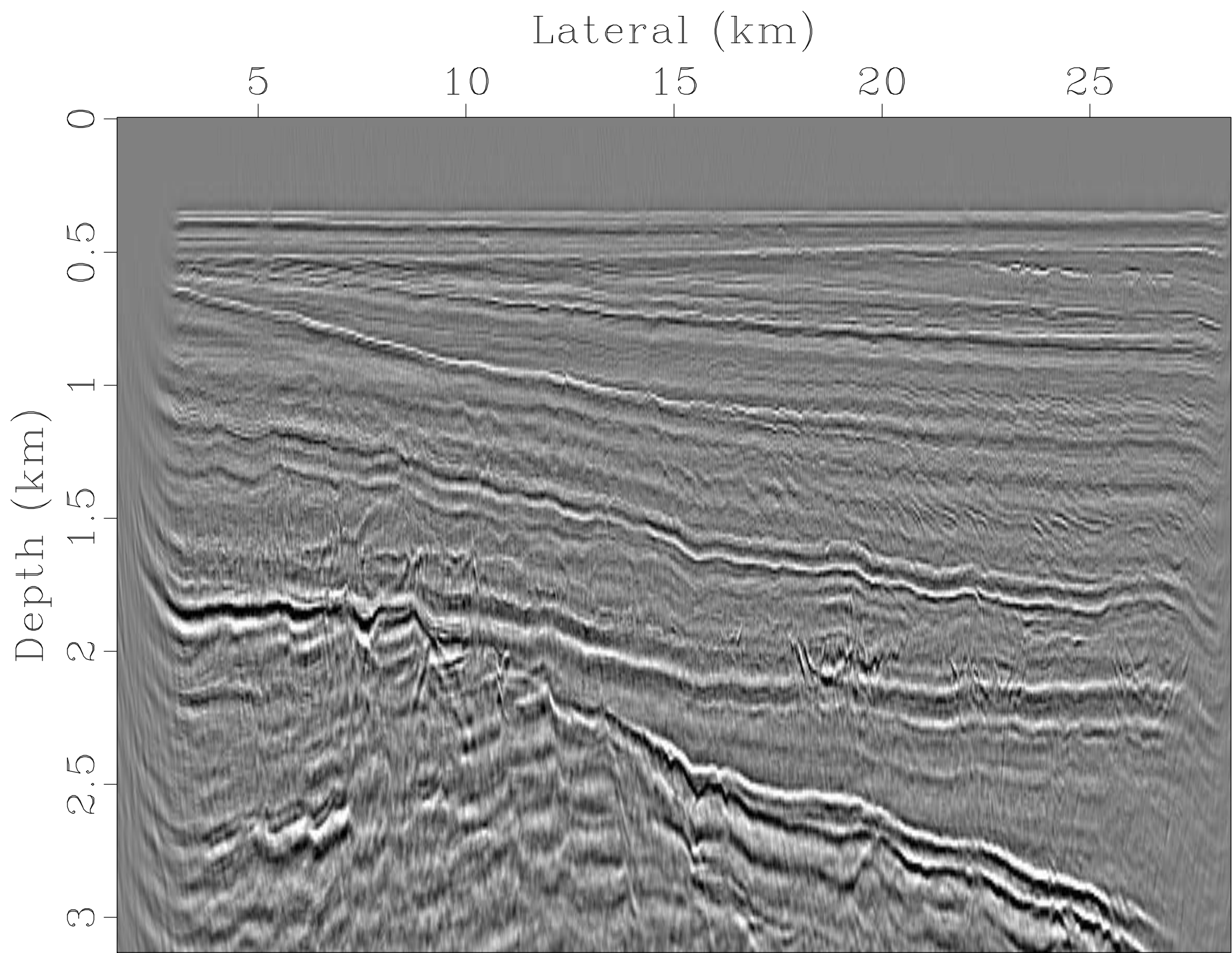
Kirchhoff PSDM
