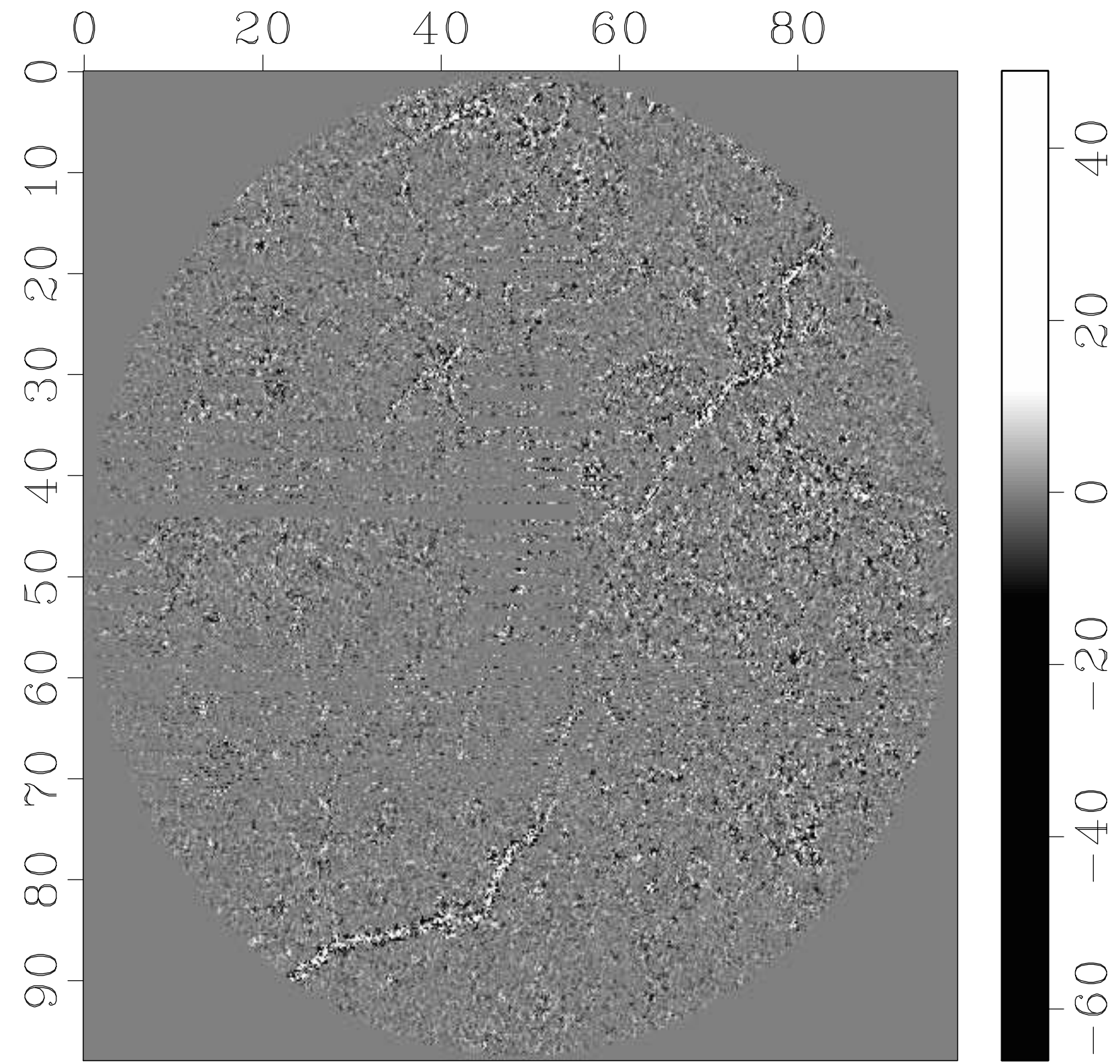
Error of Nearest Interpolation
