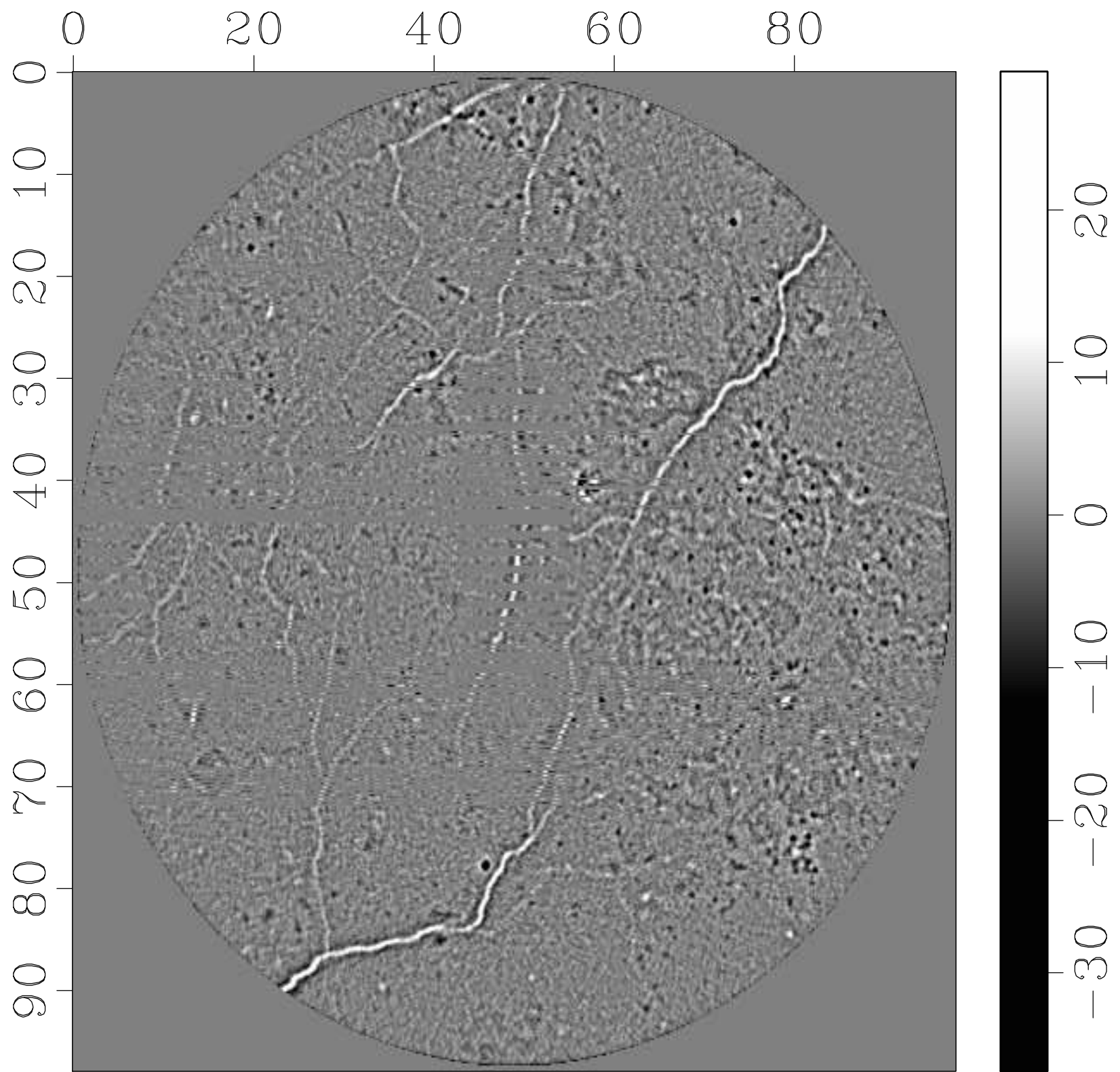
Error of Linear Interpolation
