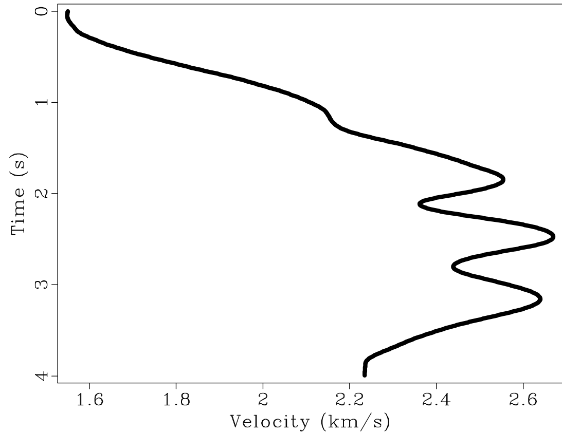
Interval Velocity
