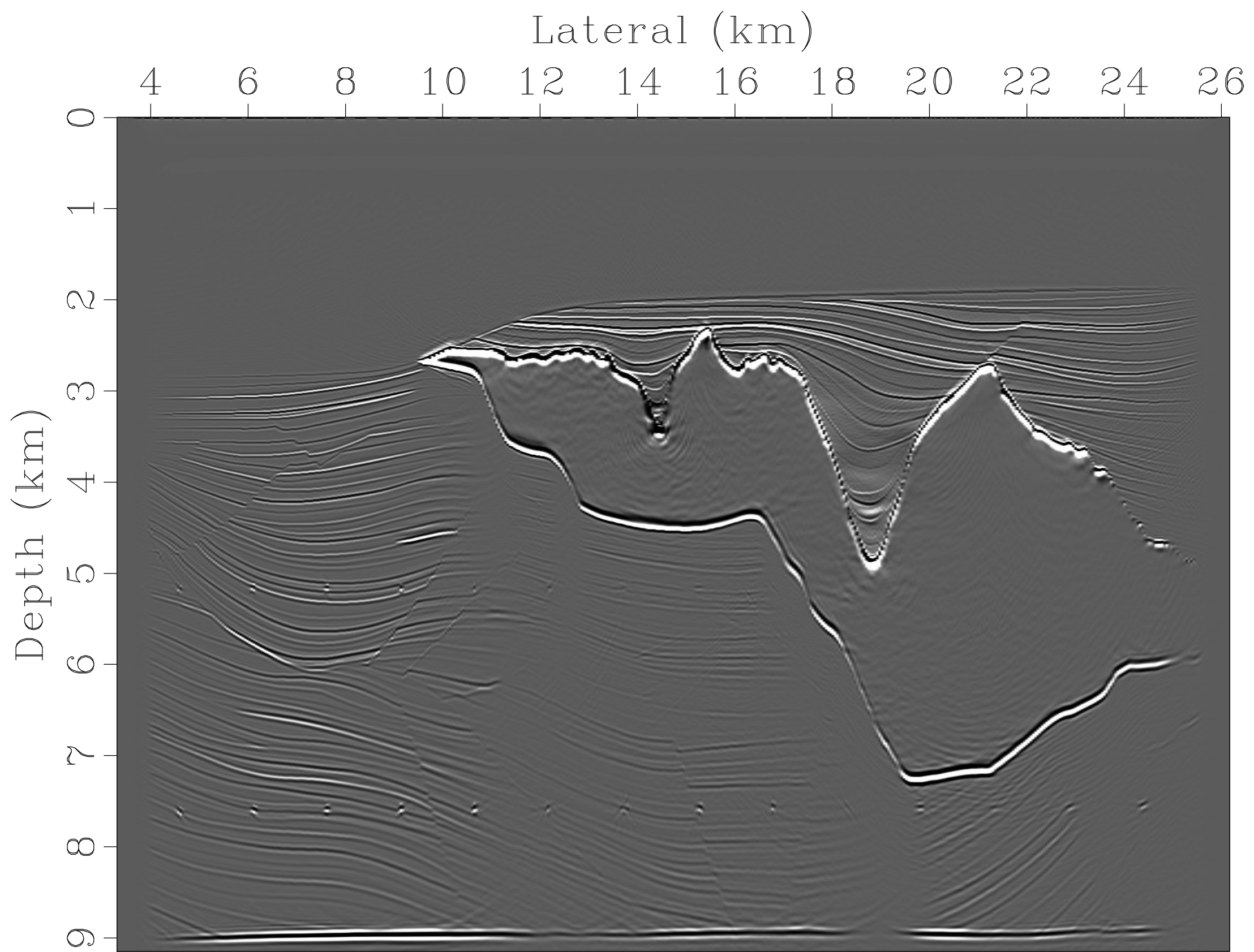
PSPI wave equation image
