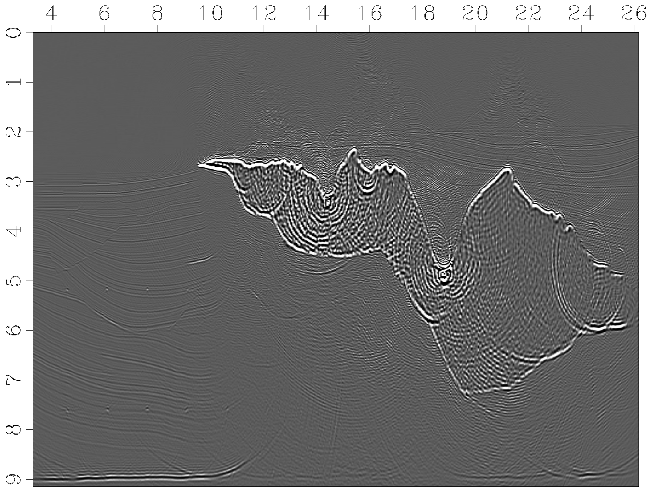
Zero-Offset Migration
