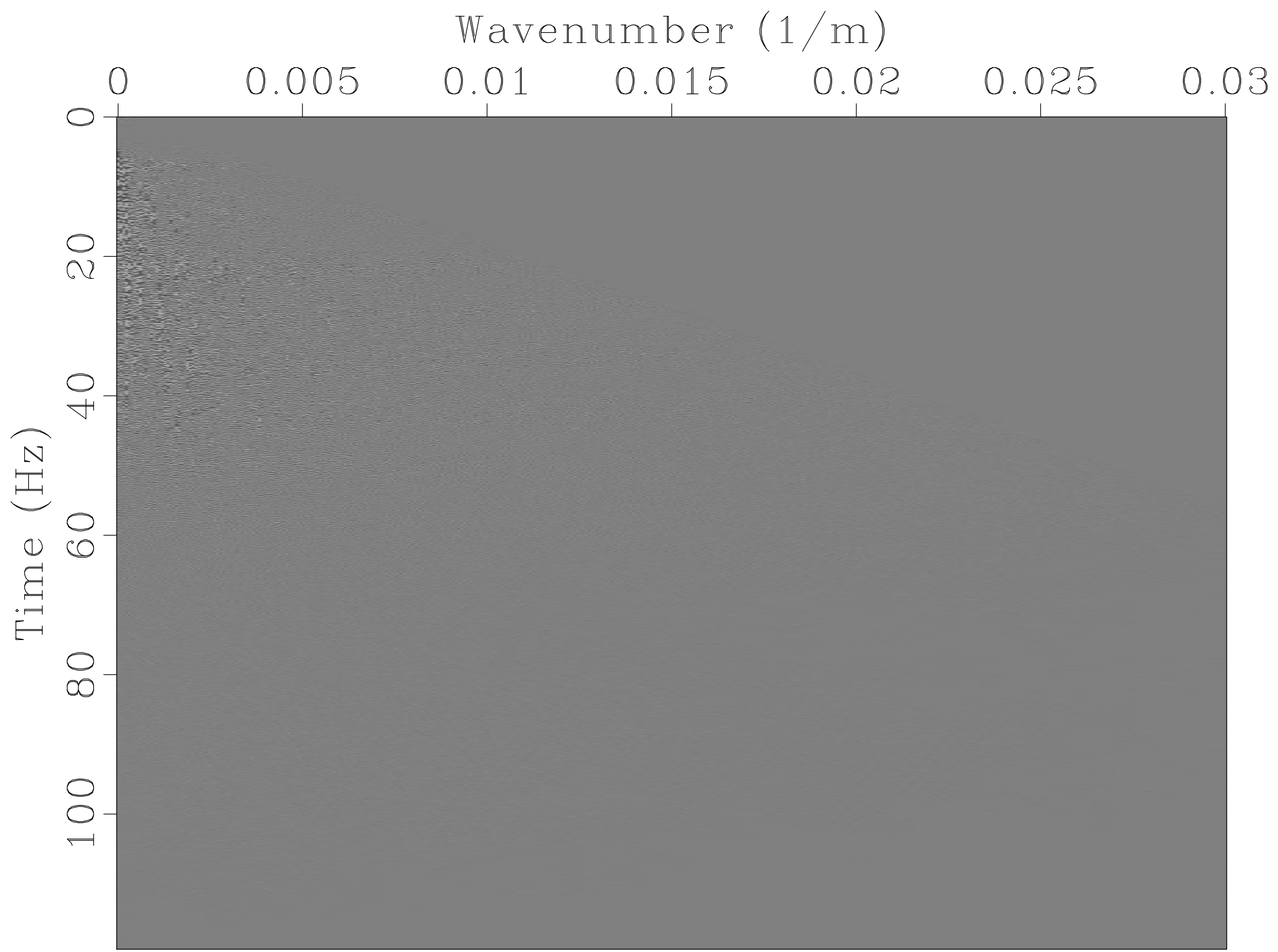
Cosine Transform Warped
