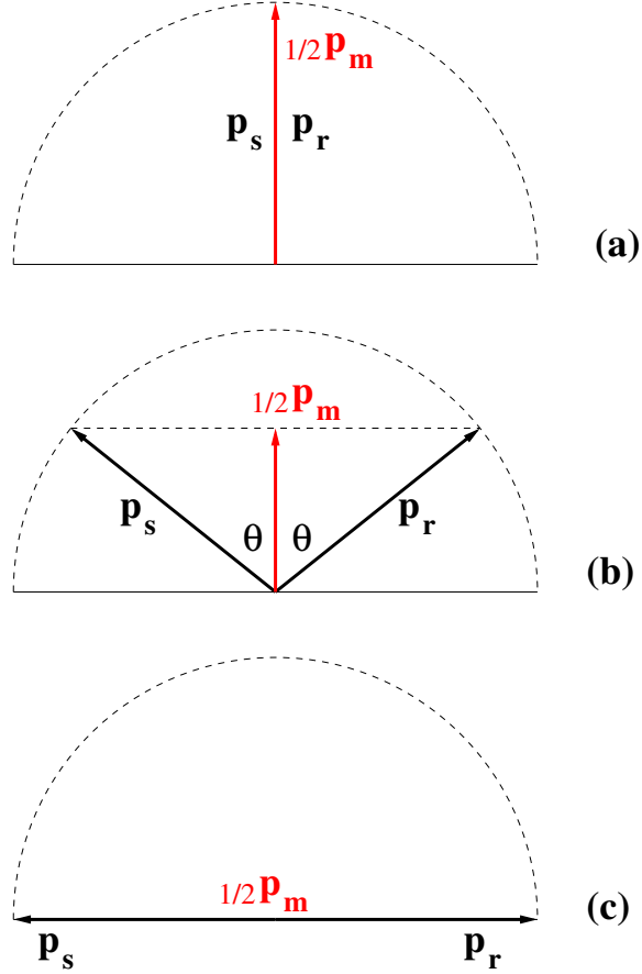
Figure 2: Interpretation of angle-decomposition based on equation (23) for time-shift gathers.
