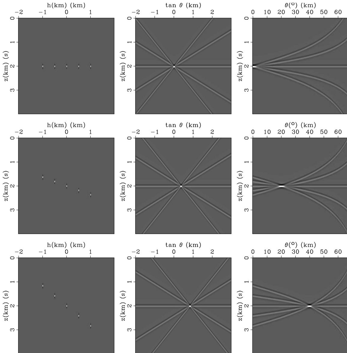
Figure 16: Image-gather formation using space-shift imaging. Each row depicts an event at 0^{\circ} (top), 20^{\circ} (middle), and 40^{\circ} (bottom). Three columns correspond to sub-sampled space-shift gathers (left), slant-stacked gathers (middle), and angle-gathers (right).
