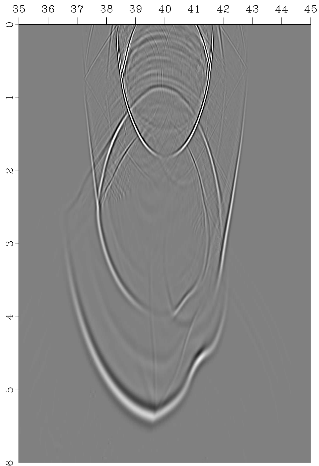
Elastic wave propagation (Z component)
