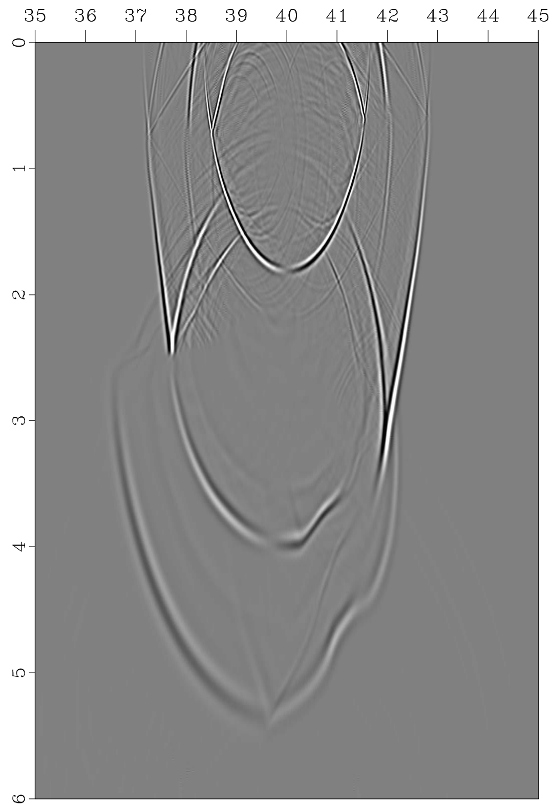
Elastic wave propagation (X component)
