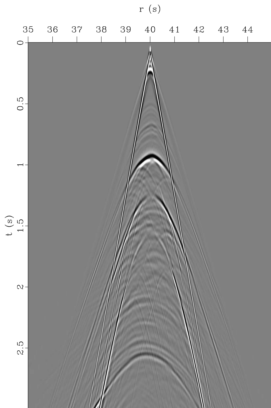
Elastic receiver data (Z component)
