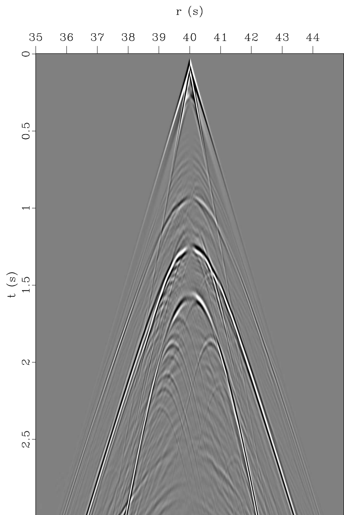
Elastic receiver data (X component)
