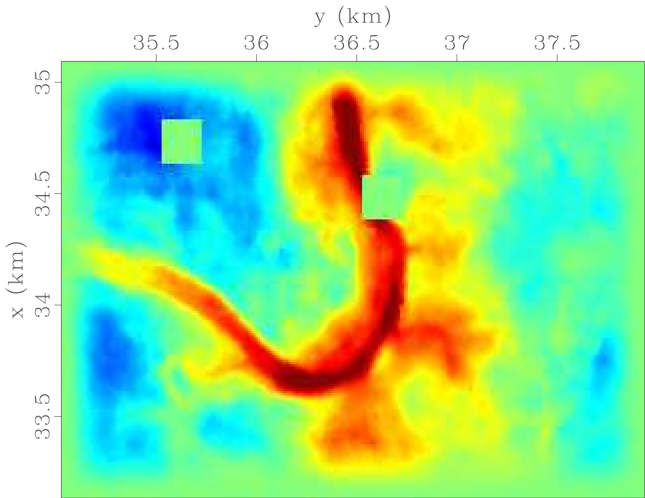
POCS interpolation (0 iterations)
