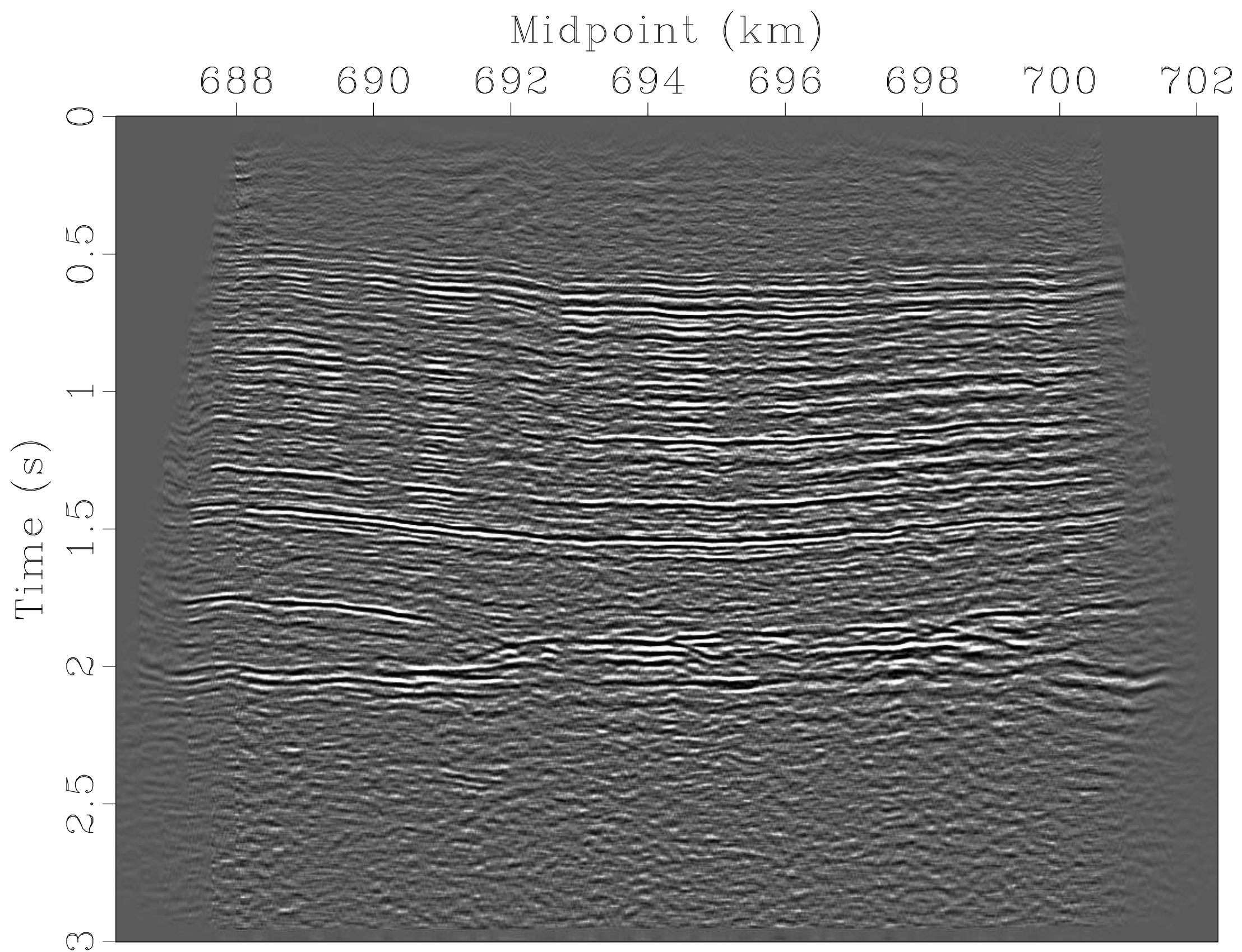
Prestack Kirchhoff Time Migration
