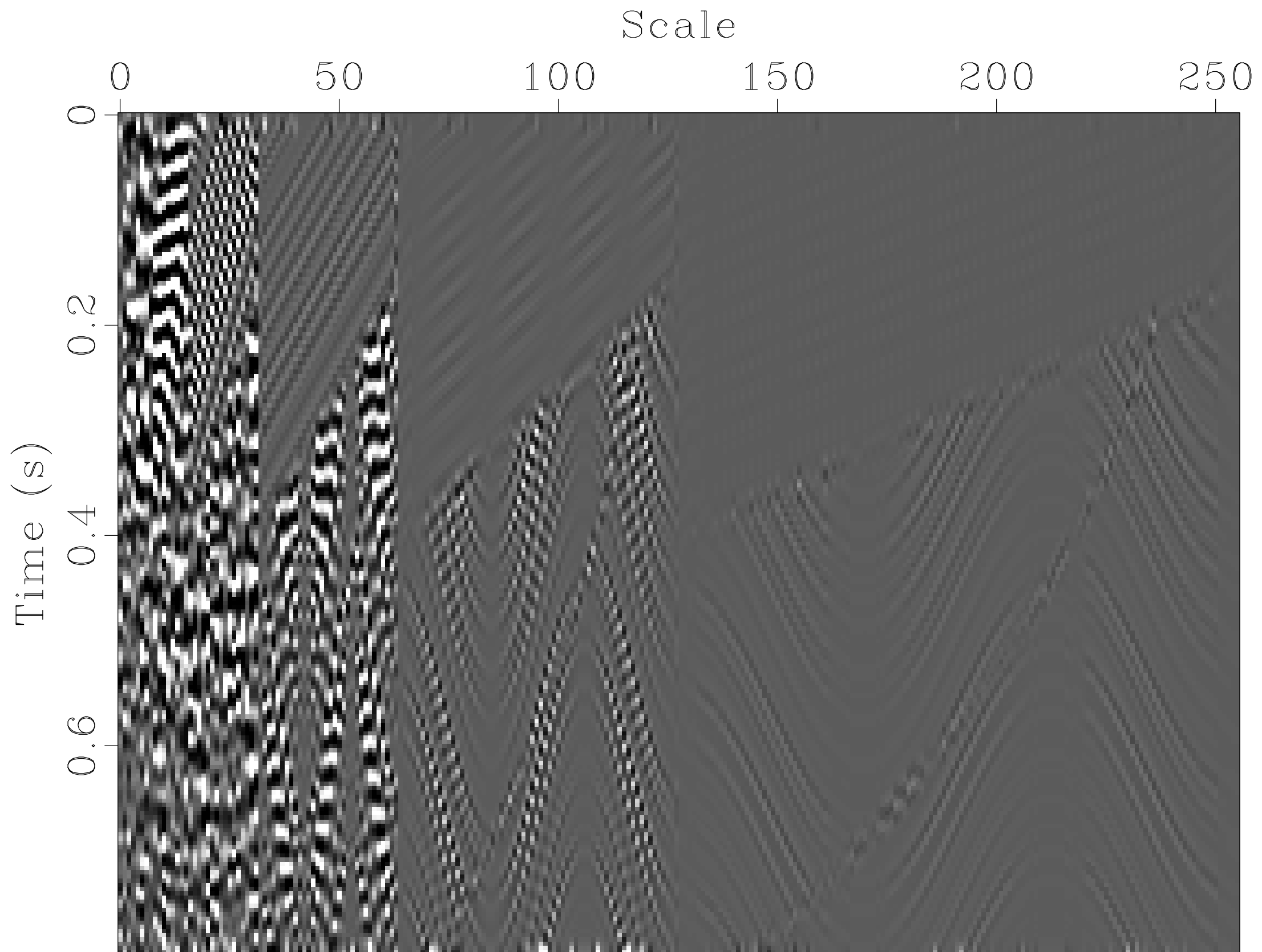
Wavelet Transform
